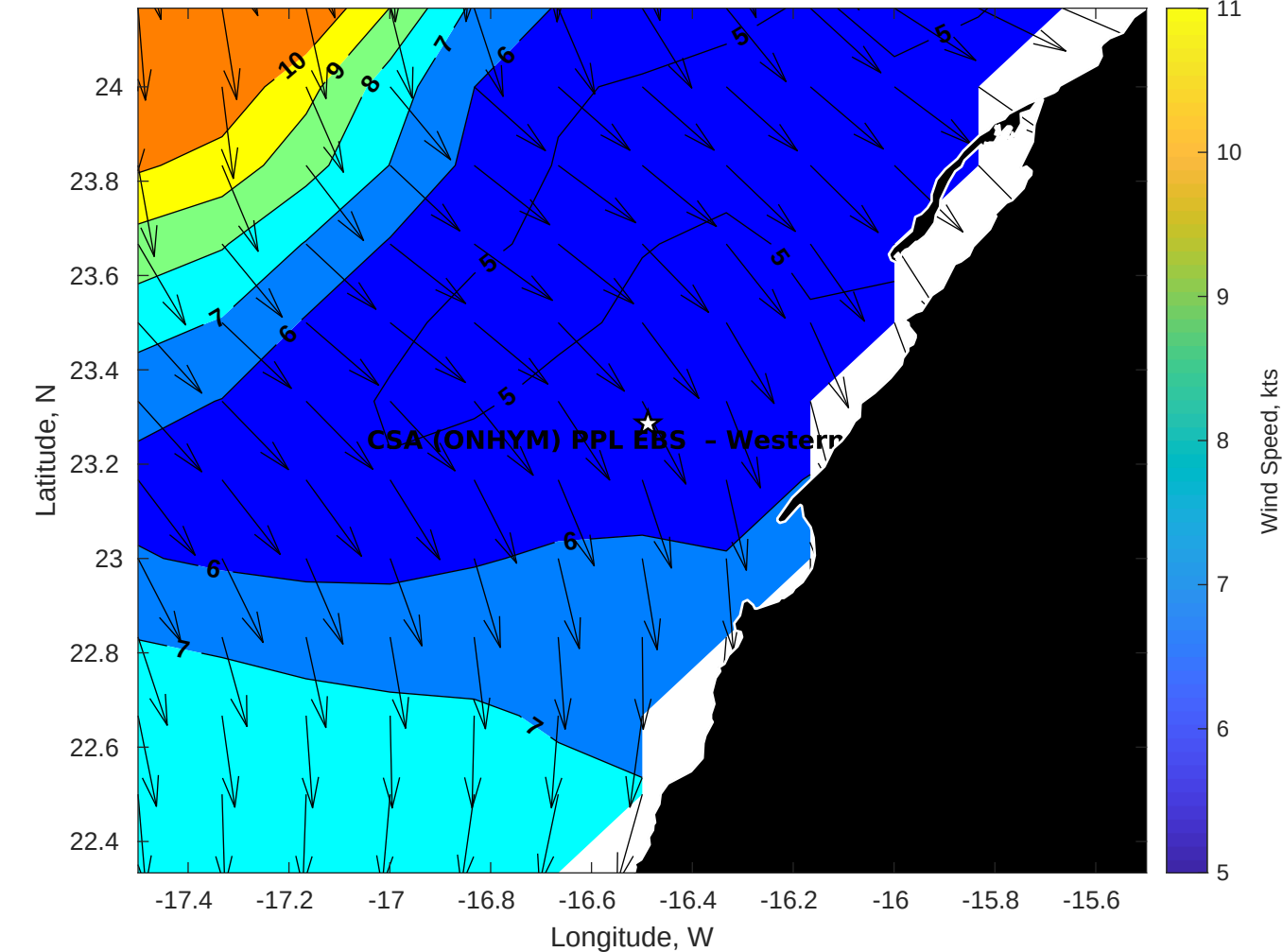
Winds (kts) for CSA (ONHYM) PPL EBS - Western Sahara at 04-Apr-2025 09:00:00
