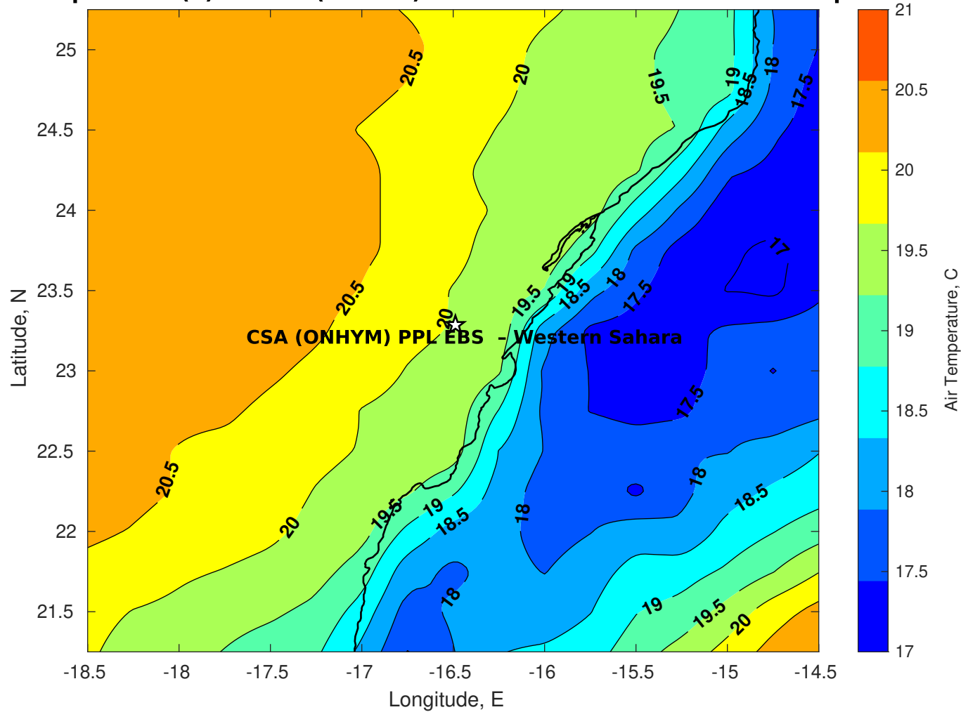
Air Temperature (C) for CSA (ONHYM) PPL EBS - Western Sahara at 04-Apr-2025
