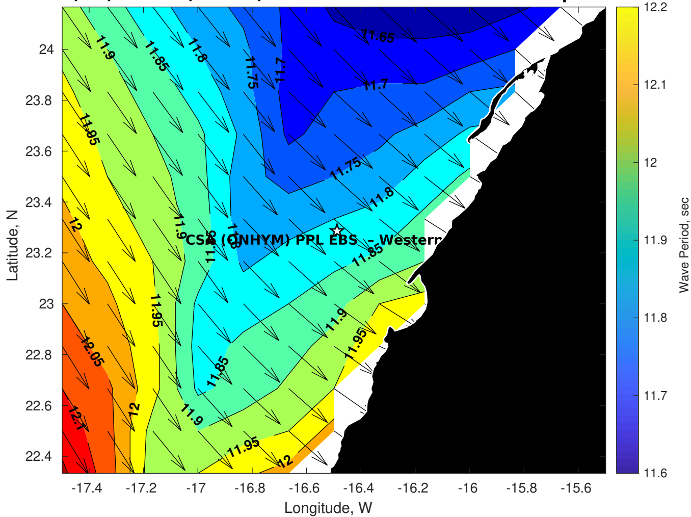
Wave Period (sec) for CSA (ONHYM) PPL EBS - Western Sahara at 04-Apr-2025 09:00:00
