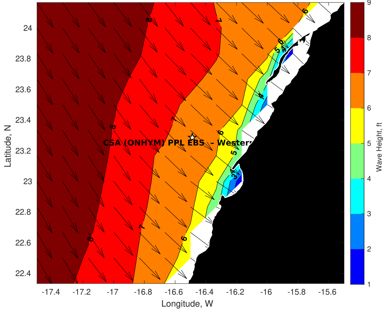
Wave Height (ft) for CSA (ONHYM) PPL EBS - Western Sahara at 04-Apr-2025 09:00:00
