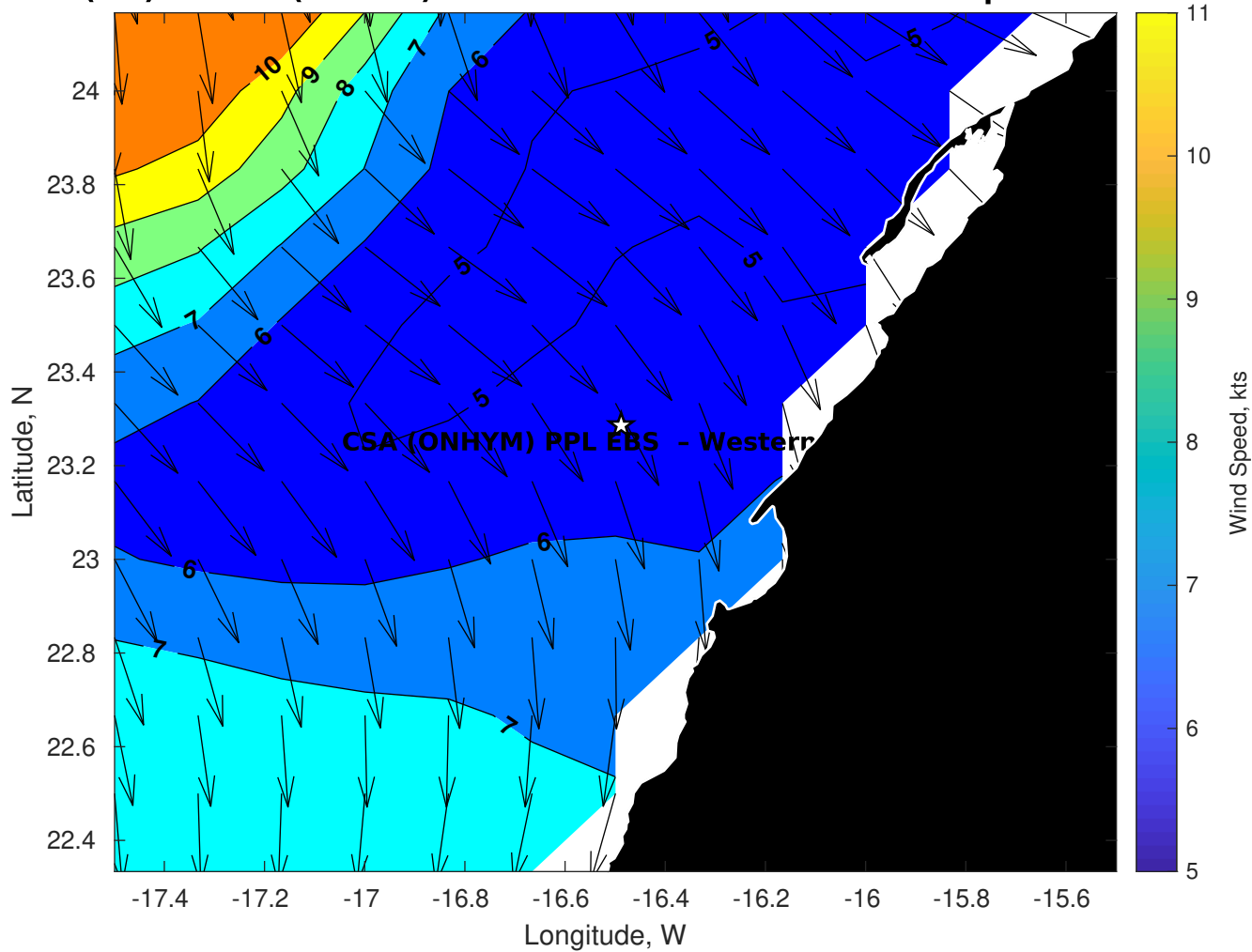
Winds (kts) for CSA (ONHYM) PPL EBS - Western Sahara at 04-Apr-2025 09:00:00
