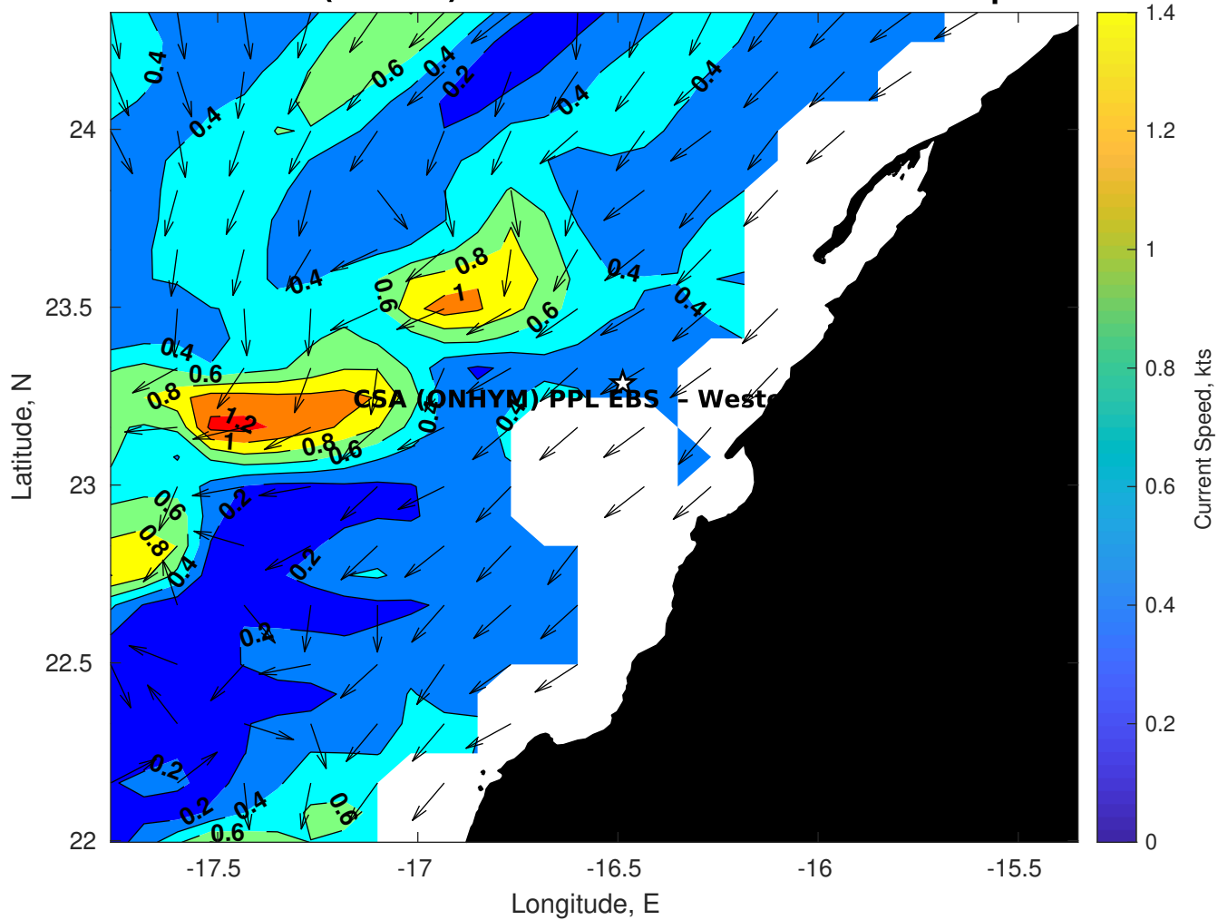
Surface Currents for CSA (ONHYM) PPL EBS - Western Sahara at 03-Apr-2025 00:00:00
