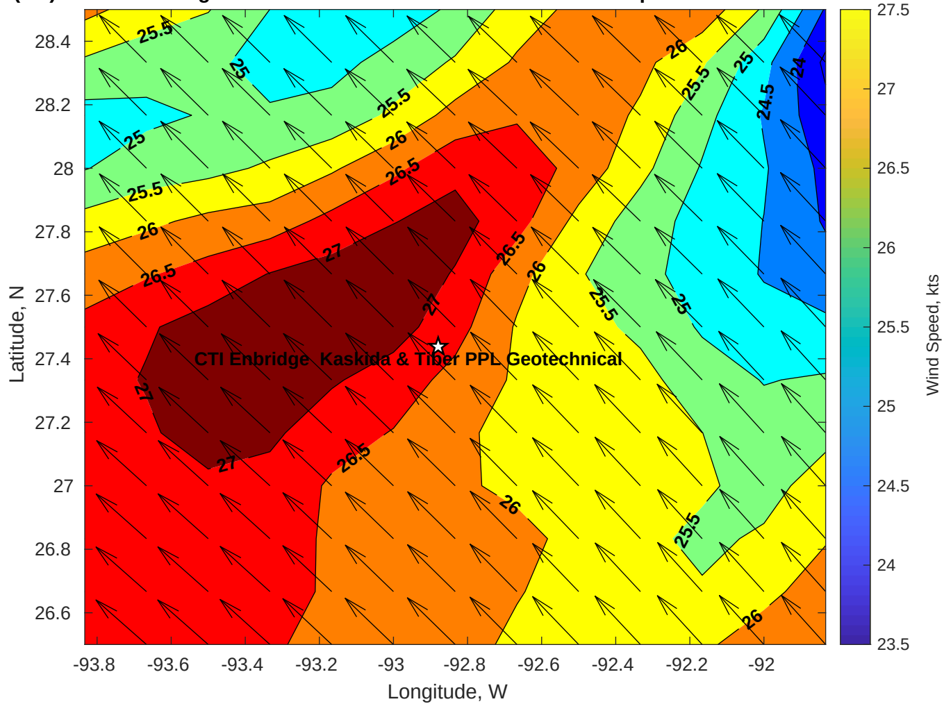
Winds (kts) for CTI Enbridge Kaskida & Tiber PPL Geotechnical at 04-Apr-2025 09:00:00
