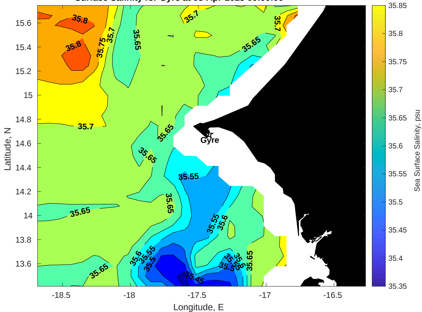
Surface Salinity for Gyre at 03-Apr-2025 00:00:00
