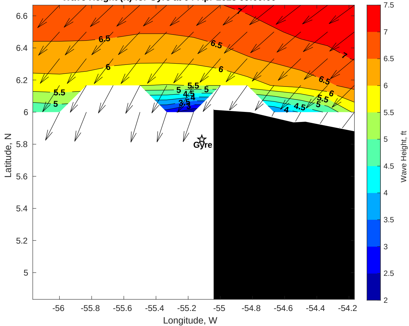
Wave Height (ft) for Gyre at 04-Apr-2025 09:00:00
