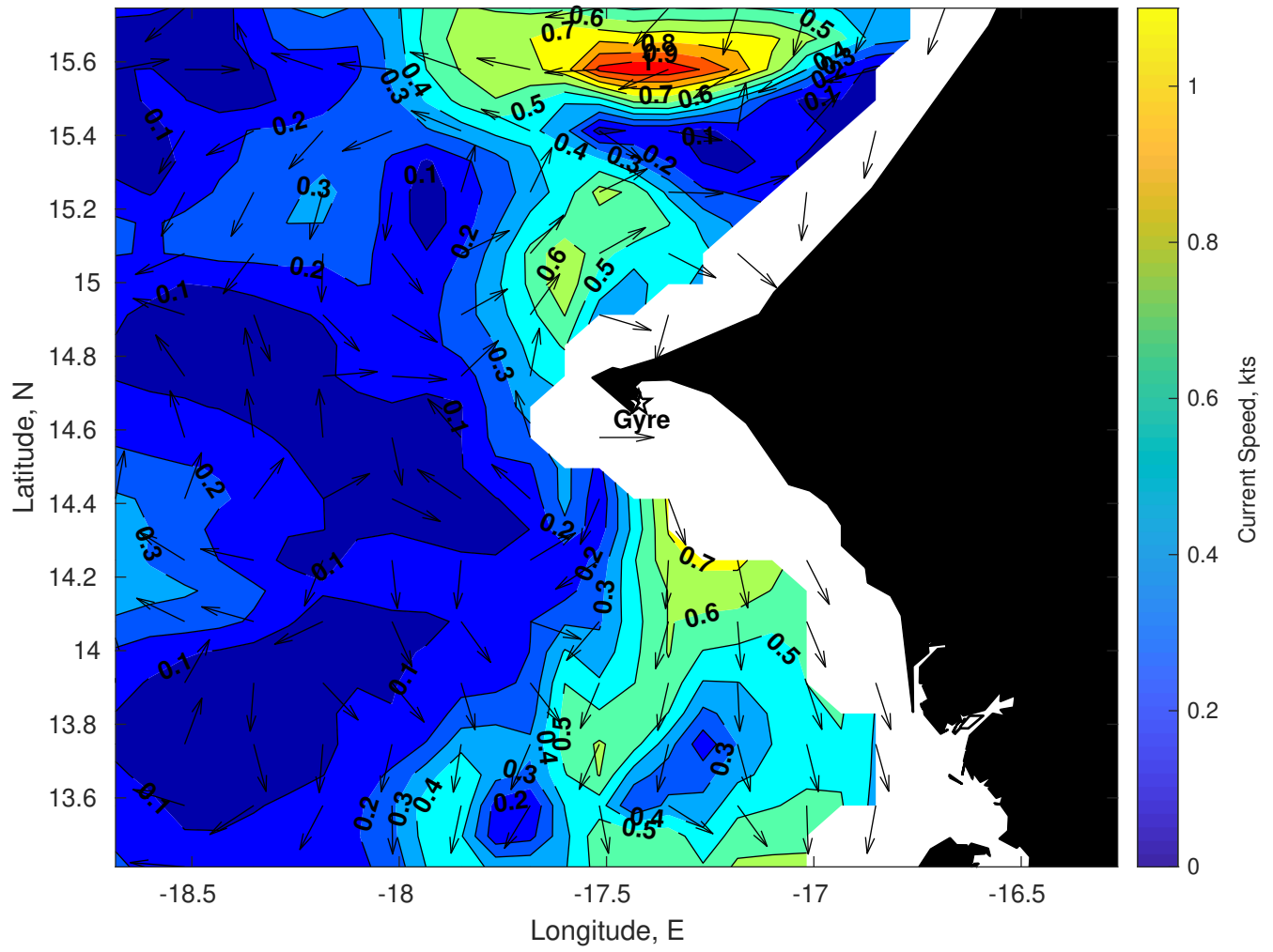
Surface Currents for Gyre at 03-Apr-2025 00:00:00
