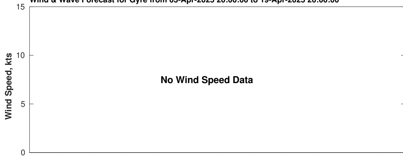
Wind & Wave Forecast for Gyre from 03-Apr-2025 20:00:00 to 19-Apr-2025 20:00:00
