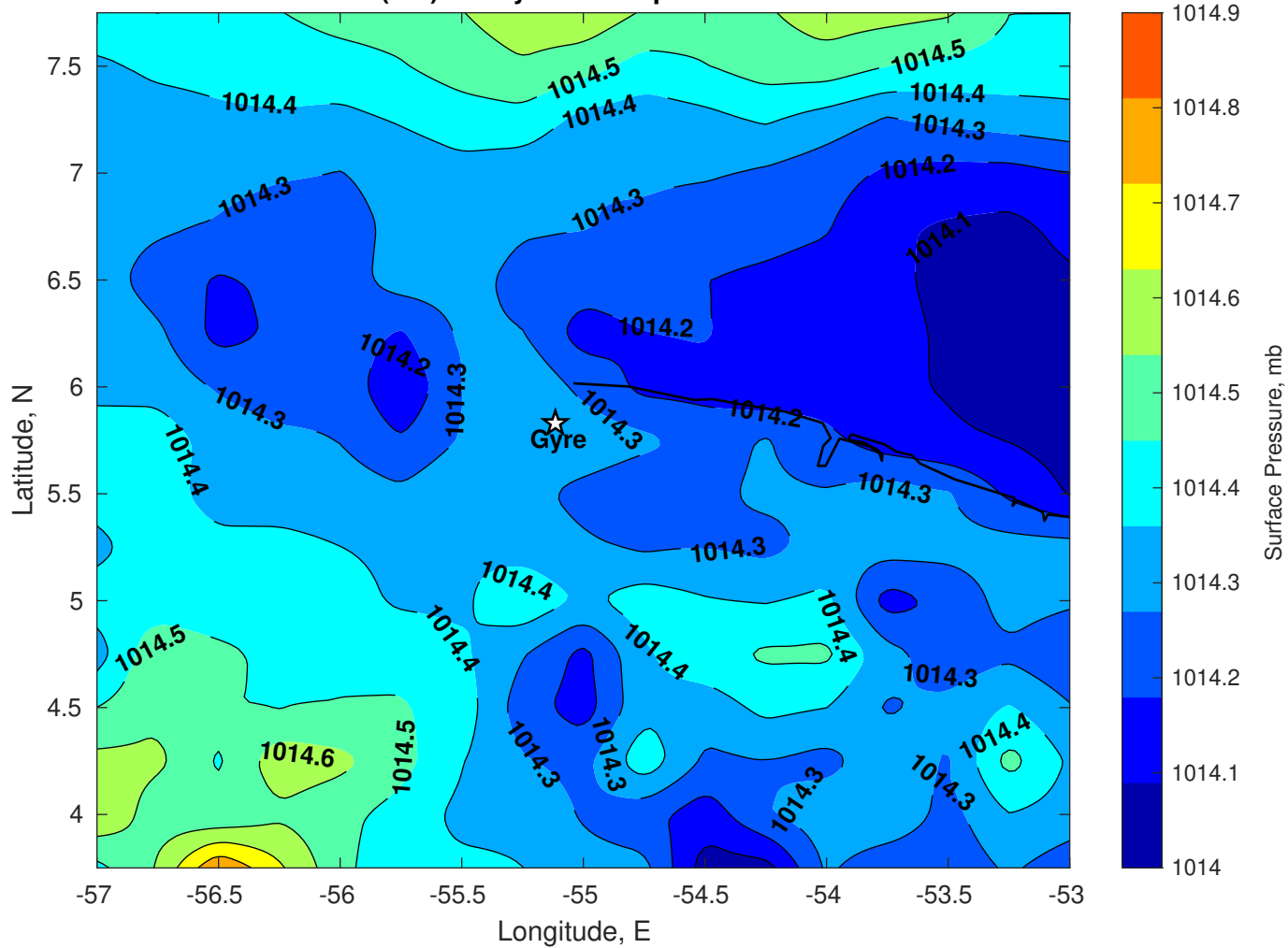
Surface Pressure (mb) for Gyre at 05-Apr-2025 00:00:00
