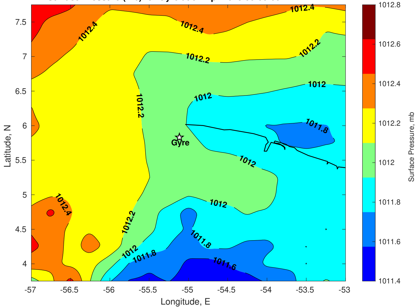
Surface Pressure (mb) for Gyre at 04-Apr-2025 00:00:00
