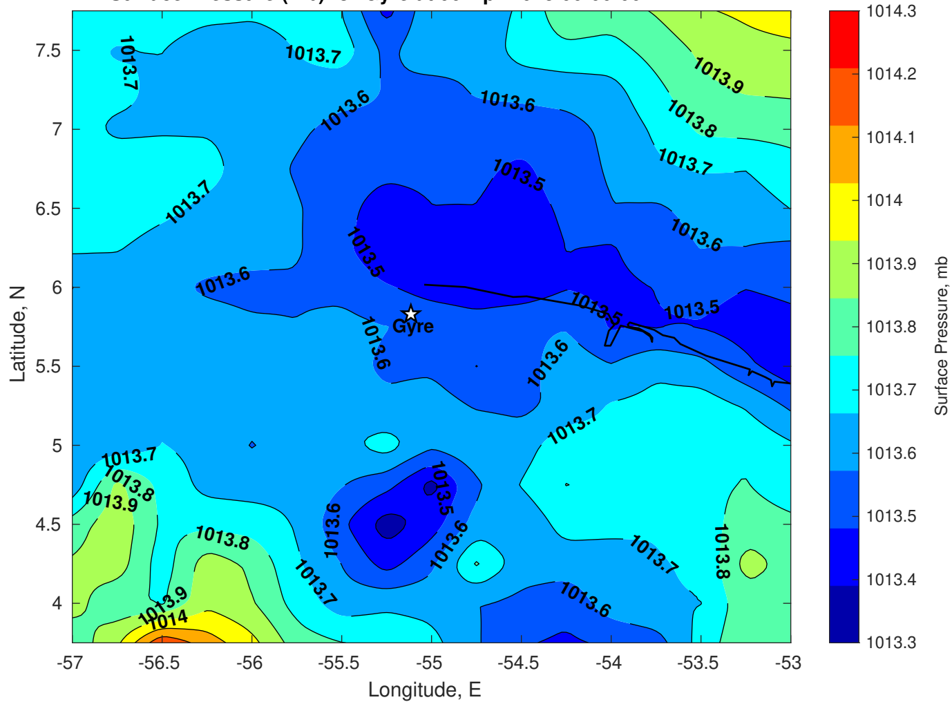
Surface Pressure (mb) for Gyre at 06-Apr-2025 00:00:00
