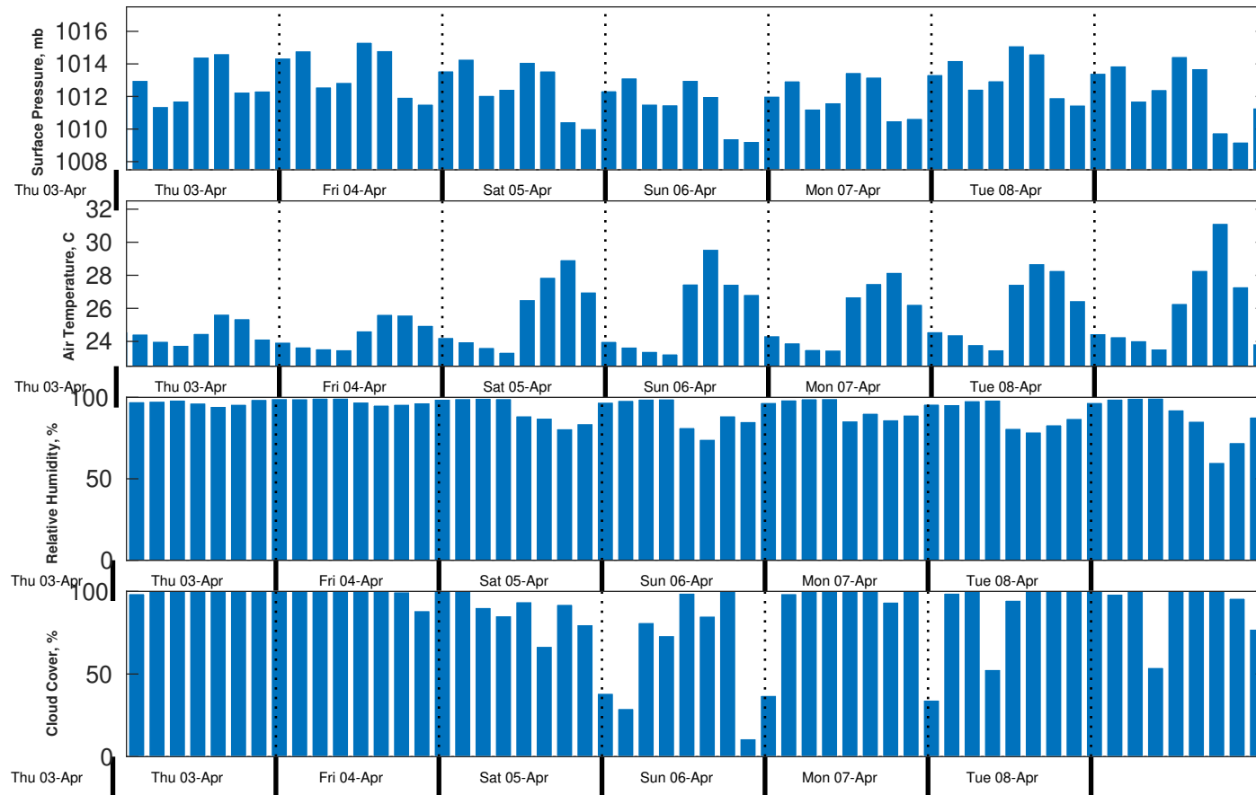
Met Forecast for Gyre from 03-Apr-2025 20:00:00 to 10-Apr-2025 20:00:00
