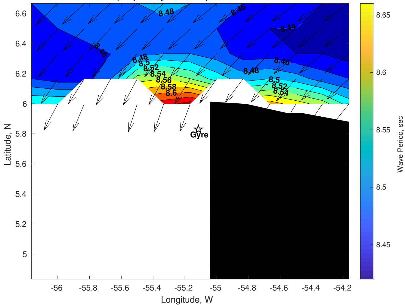
Wave Period (sec) for Gyre at 04-Apr-2025 09:00:00
