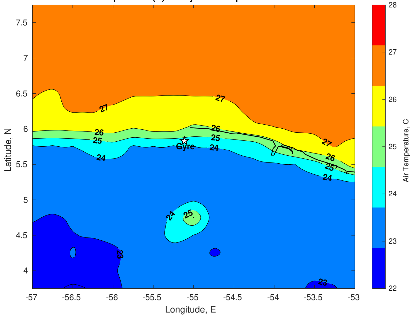
Air Temperature (C) for Gyre at 04-Apr-2025
