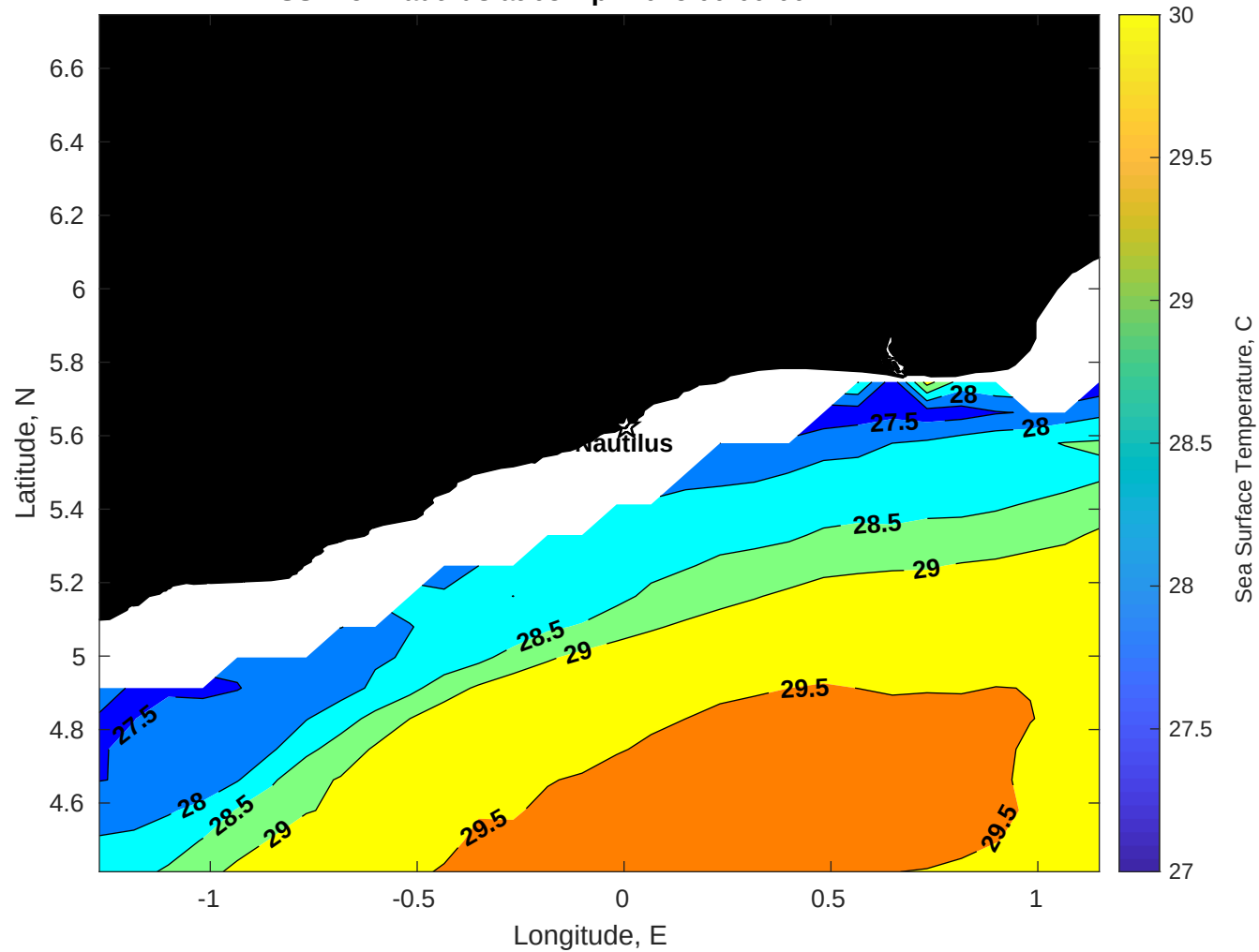
SST for Nautilus at 03-Apr-2025 00:00:00
