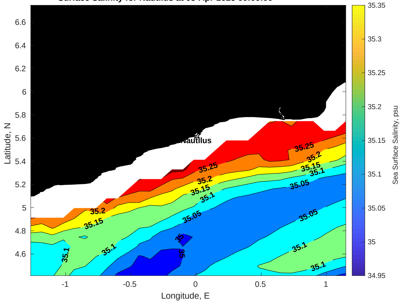
Surface Salinity for Nautilus at 03-Apr-2025 00:00:00
