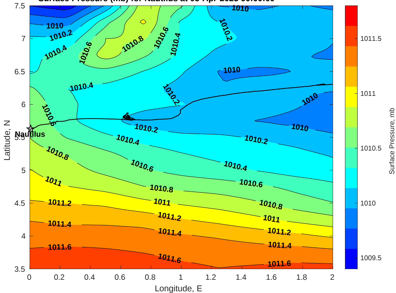
Surface Pressure (mb) for Nautilus at 05-Apr-2025 00:00:00
