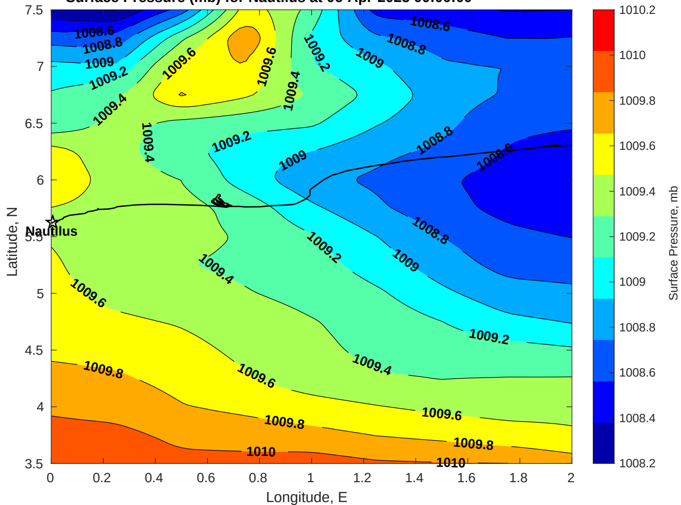
Surface Pressure (mb) for Nautilus at 06-Apr-2025 00:00:00
