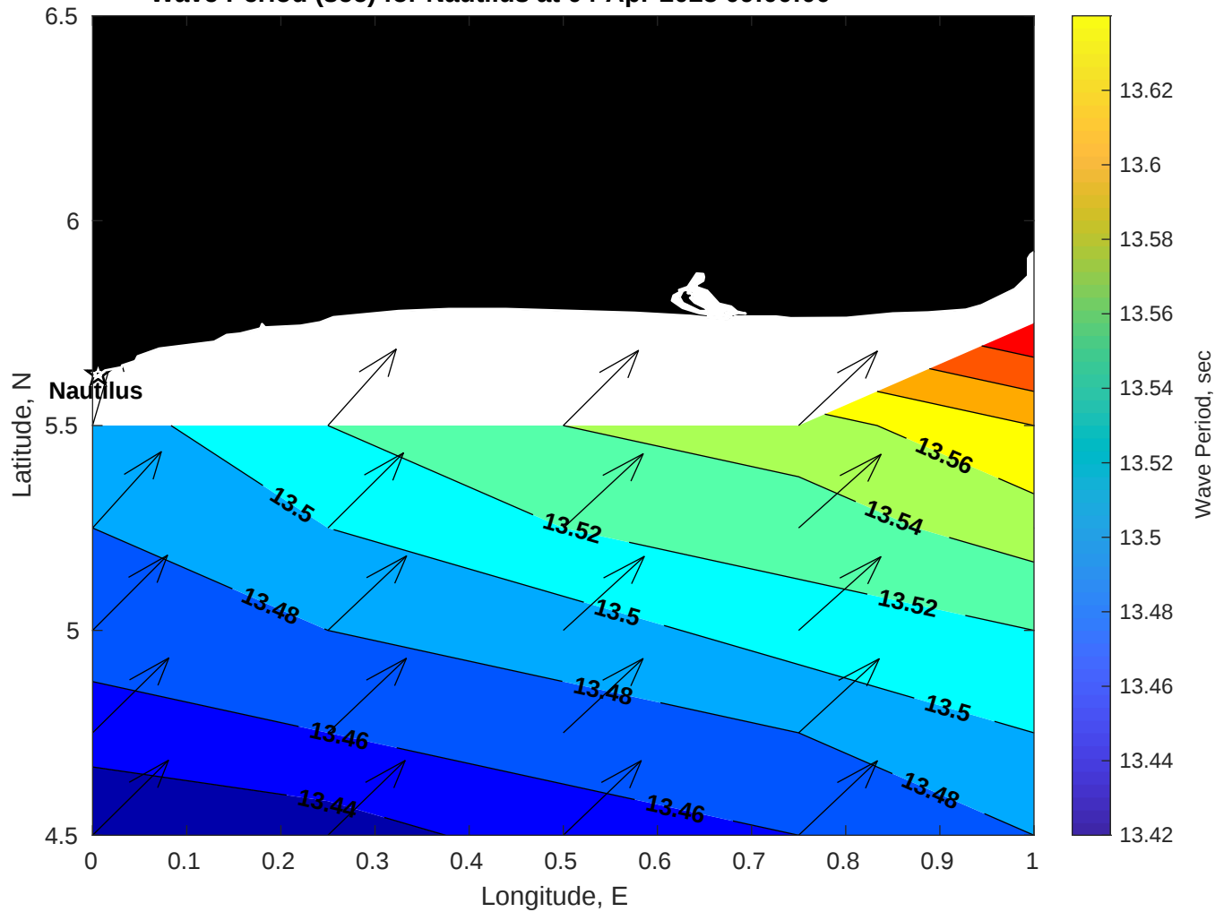
Wave Period (sec) for Nautilus at 04-Apr-2025 09:00:00
