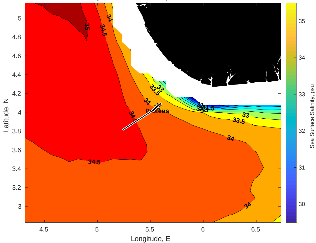
Surface Salinity for Proteus at 03-Apr-2025 00:00:00
