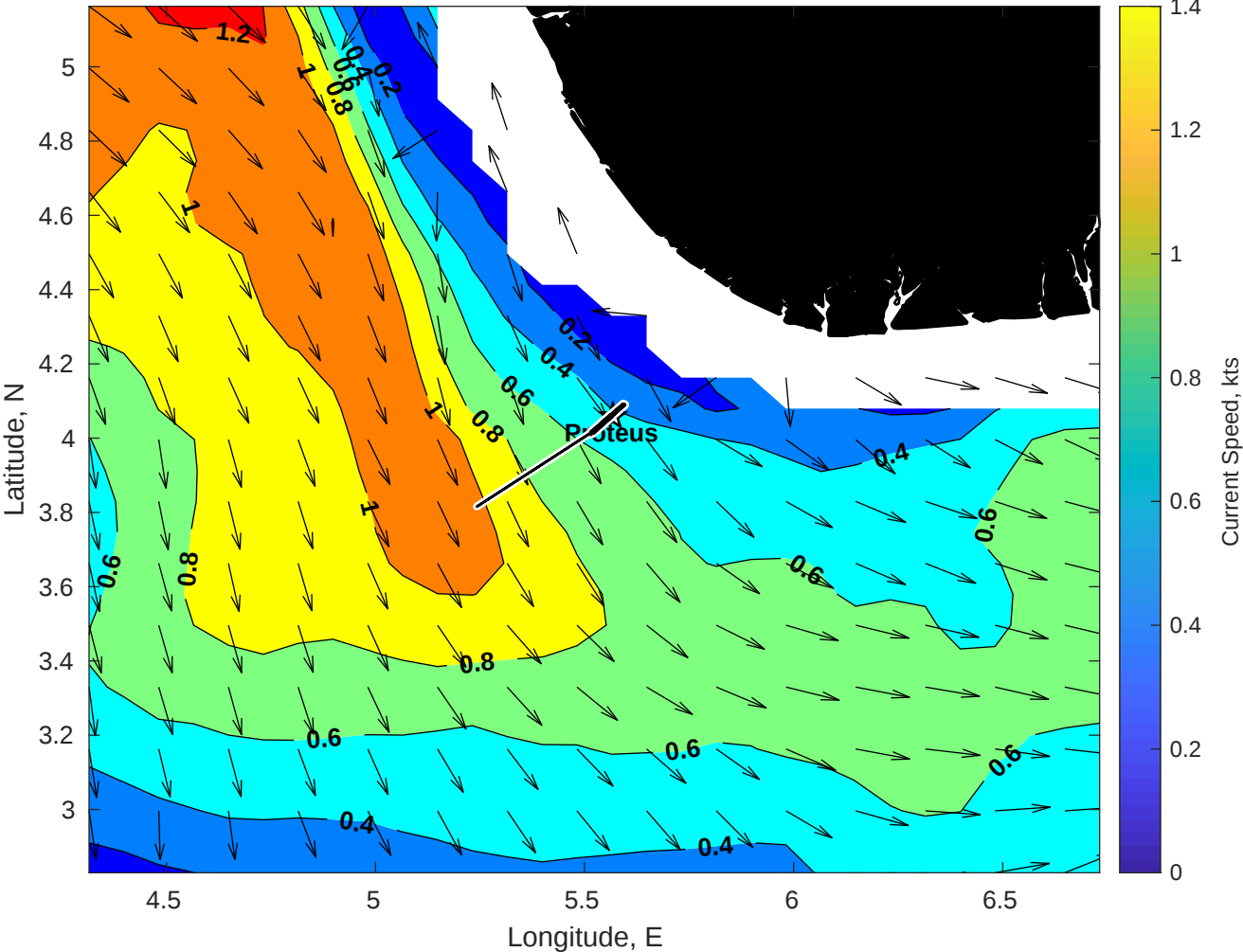
Surface Currents for Proteus at 03-Apr-2025 00:00:00
