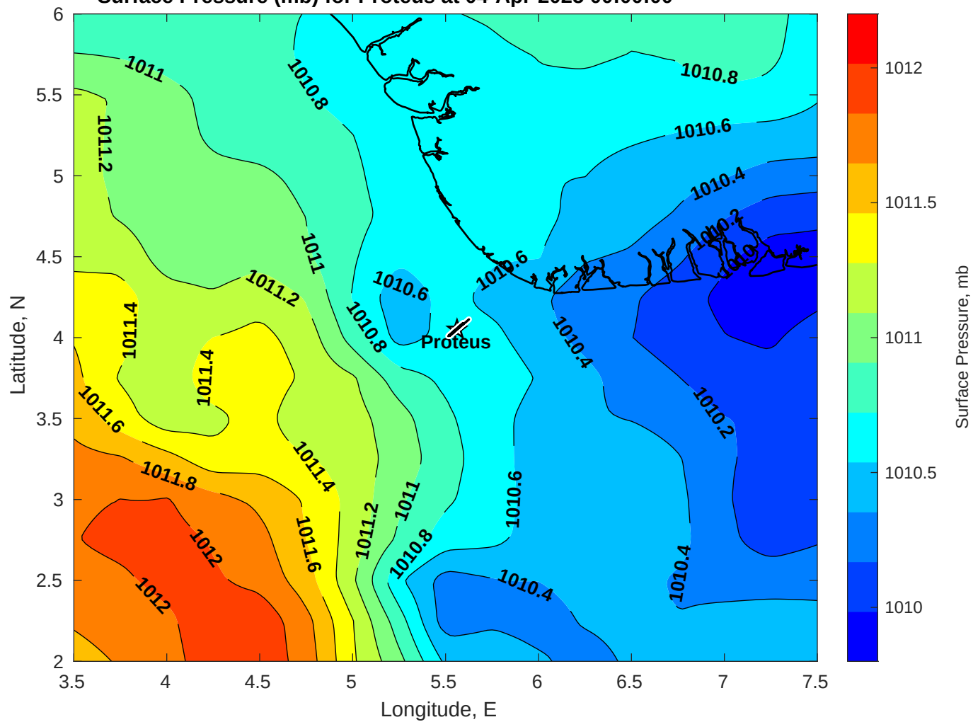
Surface Pressure (mb) for Proteus at 04-Apr-2025 00:00:00
