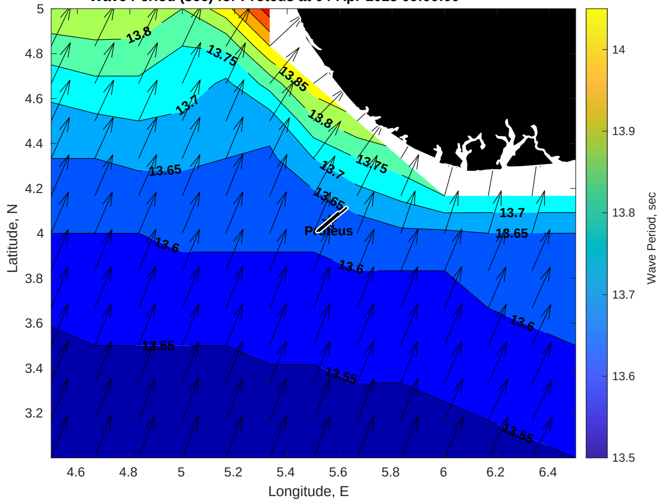
Wave Period (sec) for Proteus at 04-Apr-2025 09:00:00
