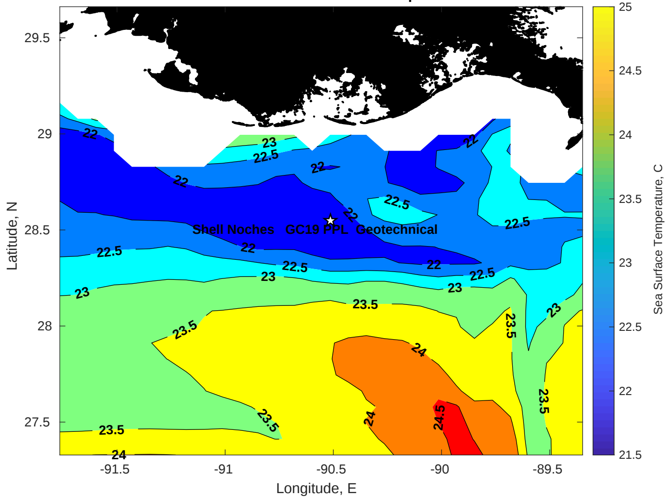
SST for Shell Noches GC19 PPL Geotechnical at 03-Apr-2025 00:00:00
