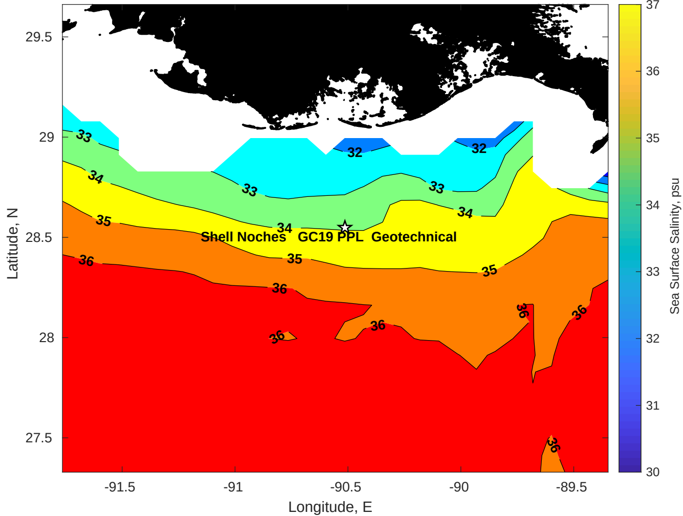
Surface Salinity for Shell Noches GC19 PPL Geotechnical at 03-Apr-2025 00:00:00
