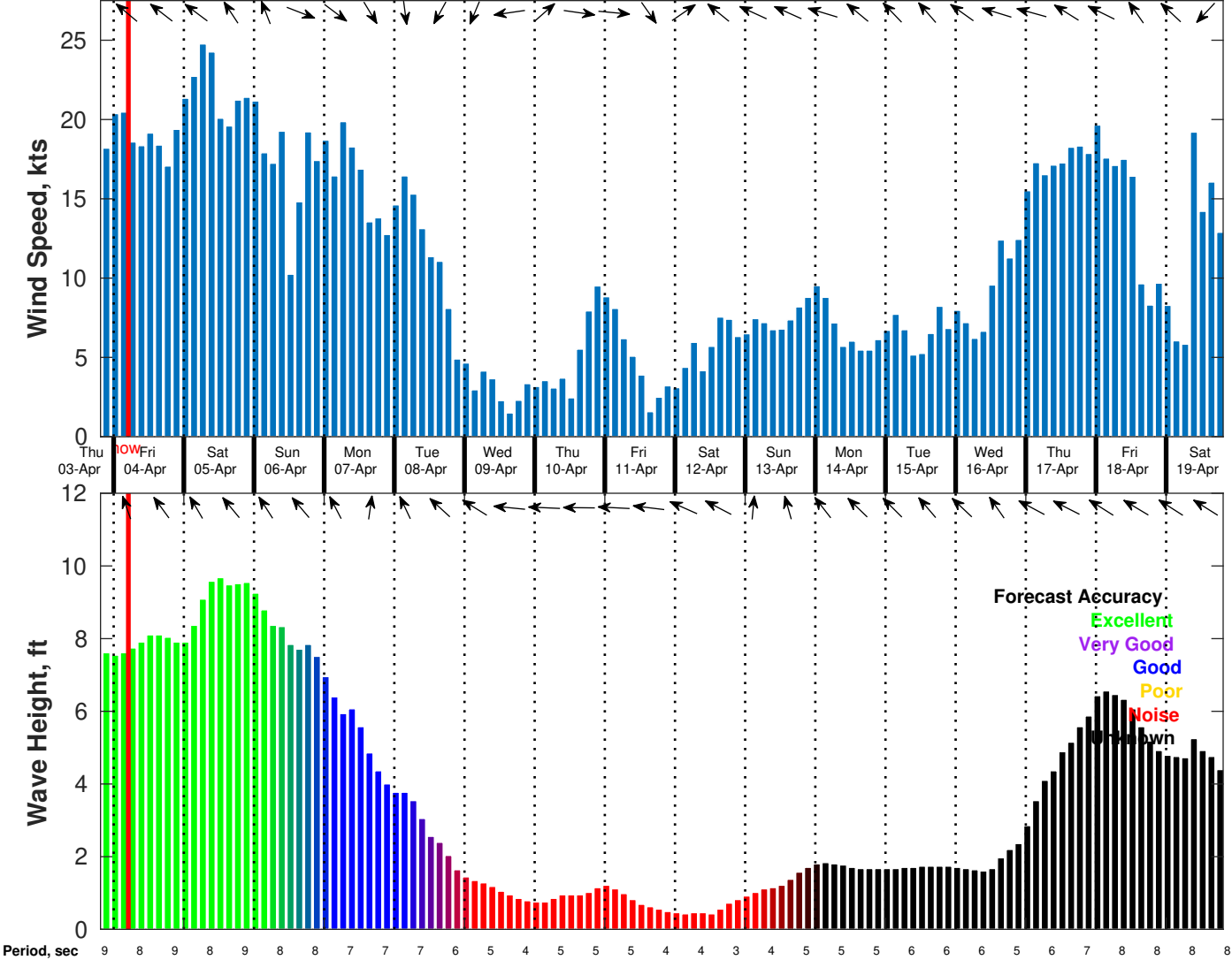
Wind & Wave Forecast for Shell Noches GC19 PPL Geotechnical from 03-Apr-2025 20:00:00 to 19-Apr-2025 20:00:00
