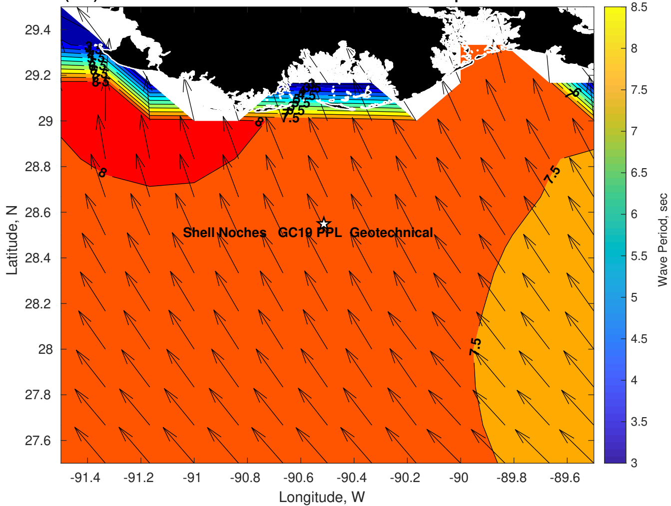
Wave Period (sec) for Shell Noches GC19 PPL Geotechnical at 04-Apr-2025 09:00:00
