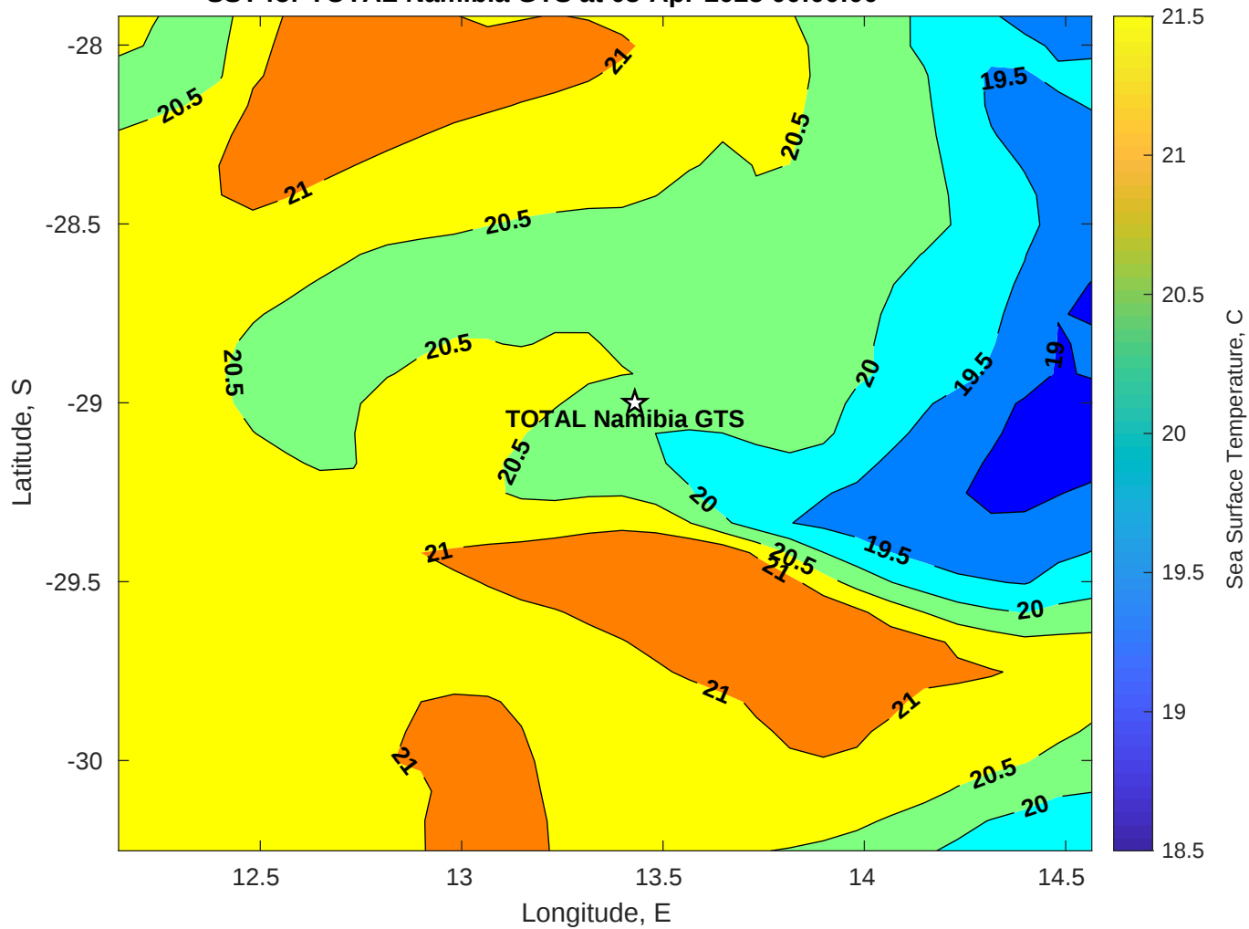
SST for TOTAL Namibia GTS at 03-Apr-2025 00:00:00
