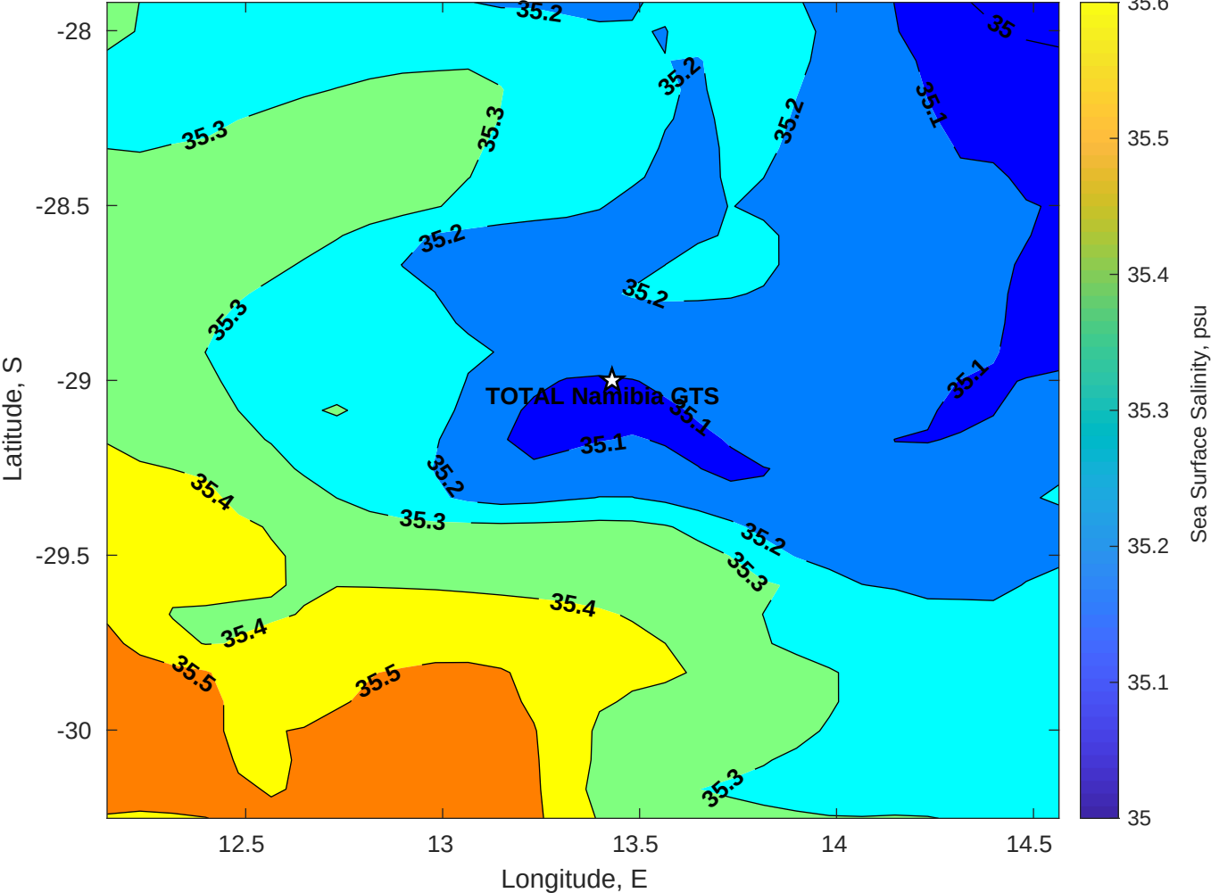
Surface Salinity for TOTAL Namibia GTS at 03-Apr-2025 00:00:00
