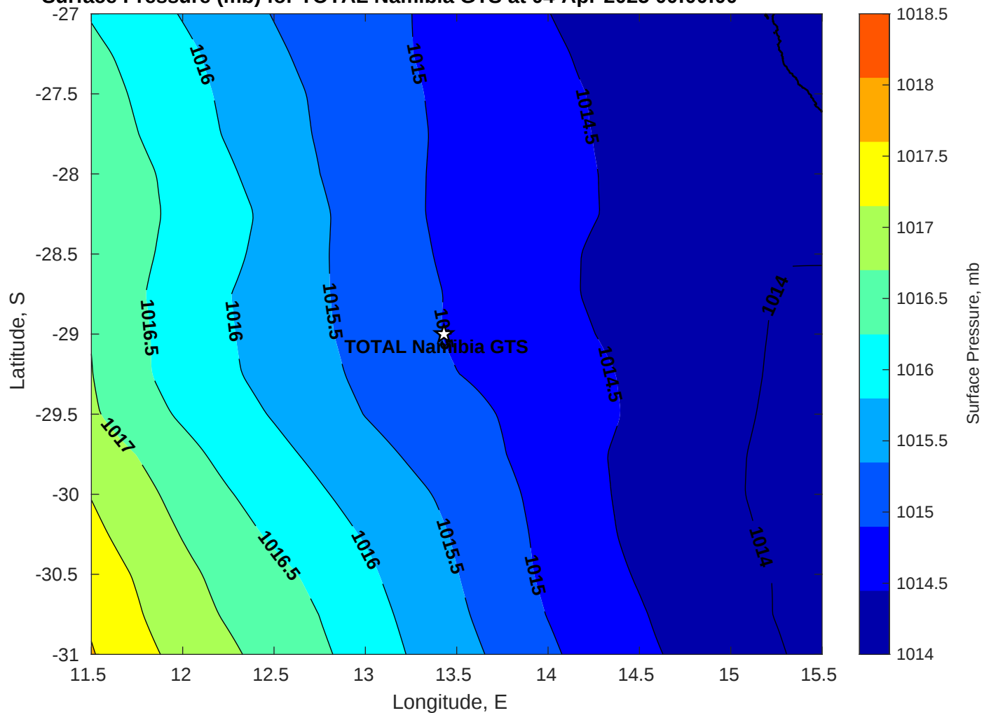
Surface Pressure (mb) for TOTAL Namibia GTS at 04-Apr-2025 00:00:00
