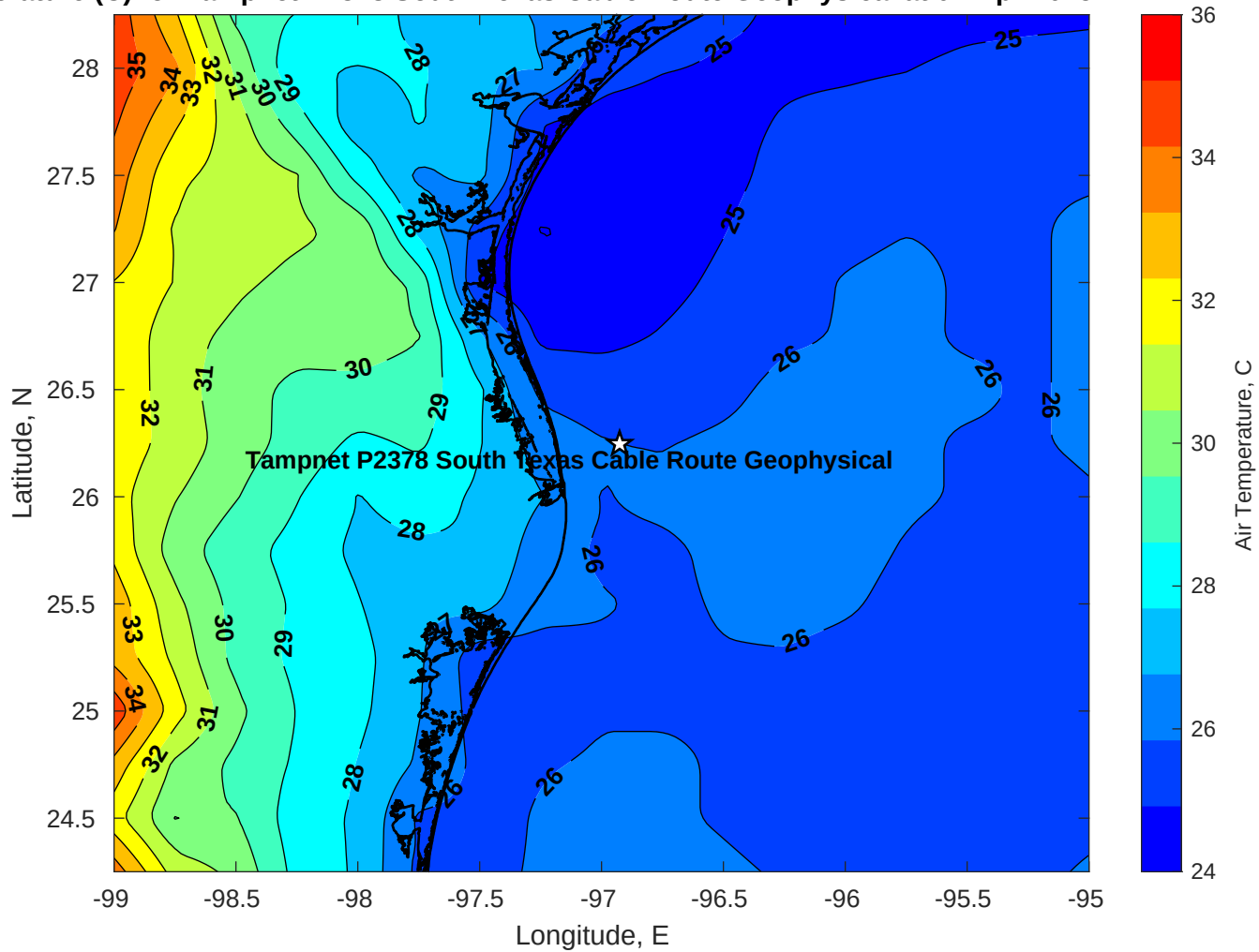
Air Temperature (C) for Tampnet P2378 South Texas Cable Route Geophysical at 04-Apr-2025
