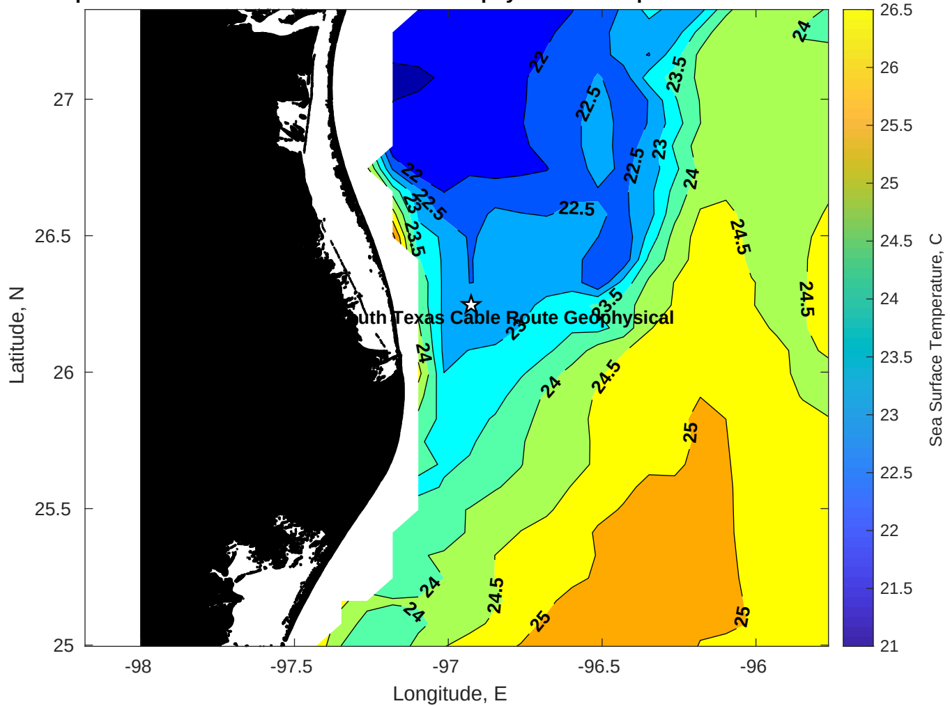
SST for Tampnet P2378 South Texas Cable Route Geophysical at 03-Apr-2025 00:00:00
