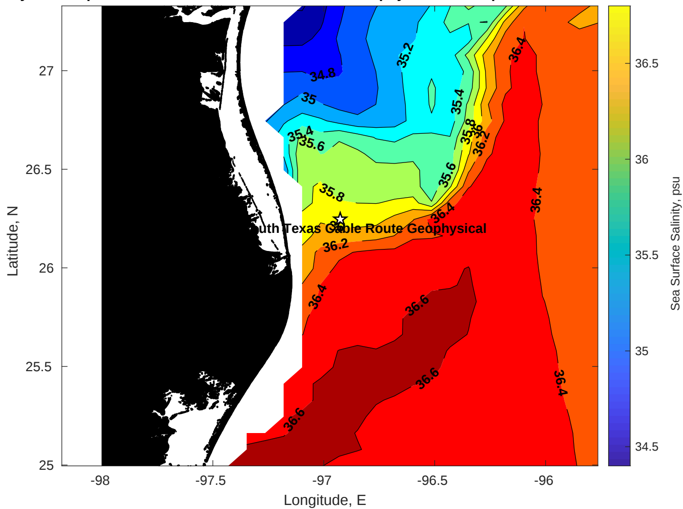
Surface Salinity for Tampnet P2378 South Texas Cable Route Geophysical at 03-Apr-2025 00:00:00
