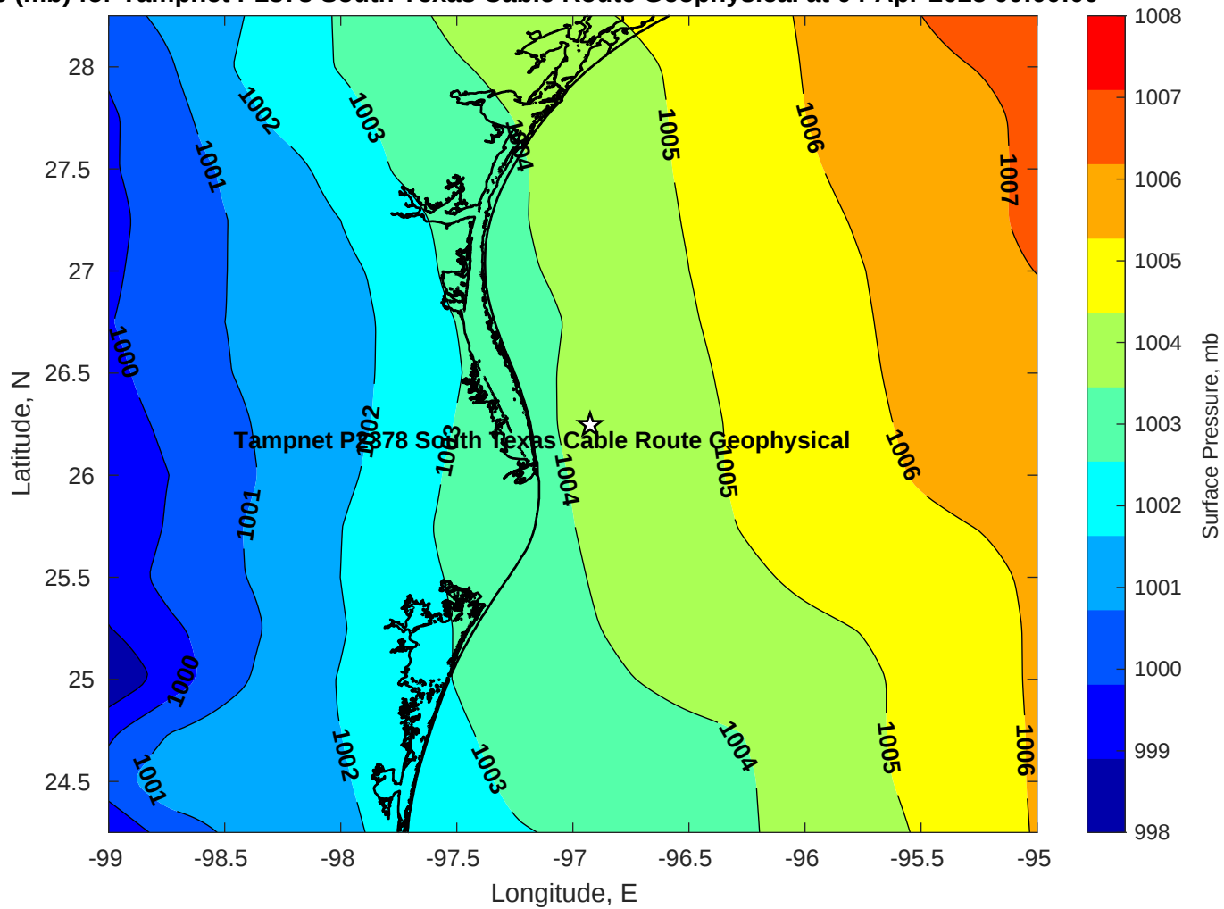
Pressure (mb) for Tampnet P2378 South Texas Cable Route Geophysical at 04-Apr-2025 00:00:00
