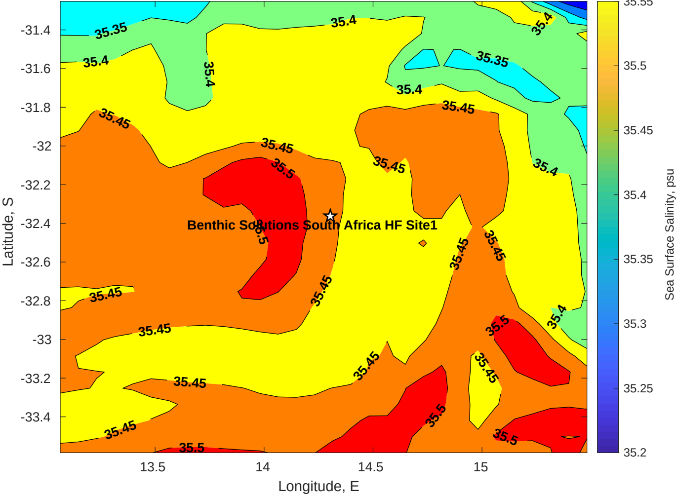
Surface Salinity for Benthic Solutions South Africa HF Site1 at 04-Apr-2025 00:00:00
