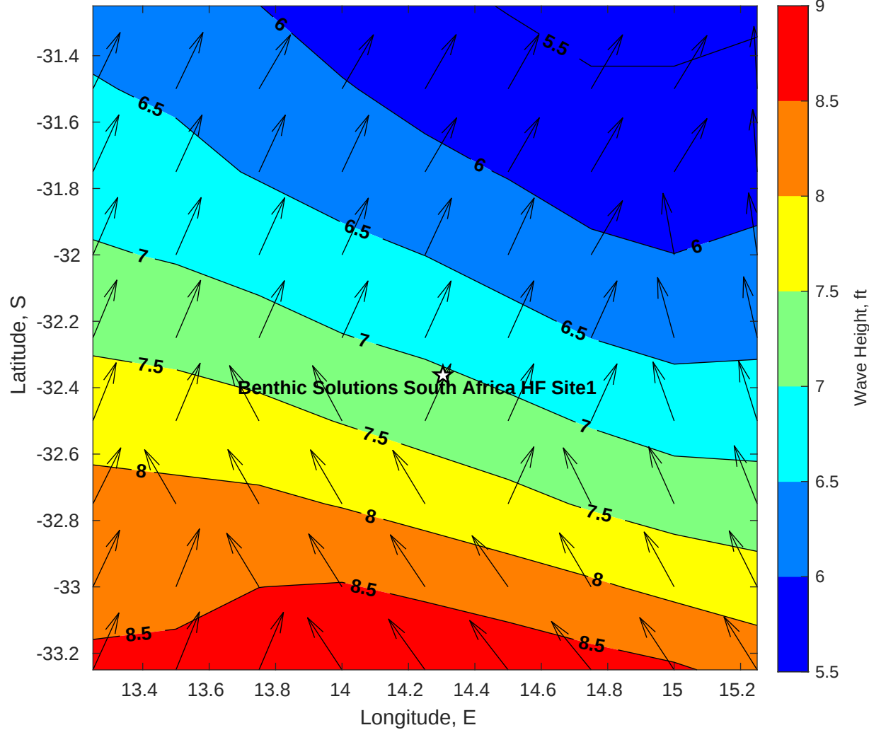
Wave Height (ft) for Benthic Solutions South Africa HF Site1 at 05-Apr-2025 09:00:00
