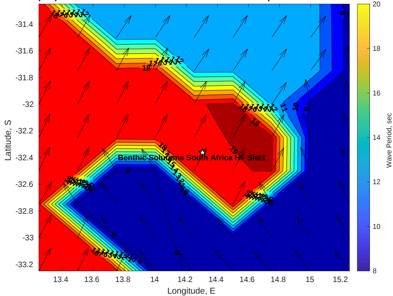
Wave Period (sec) for Benthic Solutions South Africa HF Site1 at 05-Apr-2025 09:00:00
