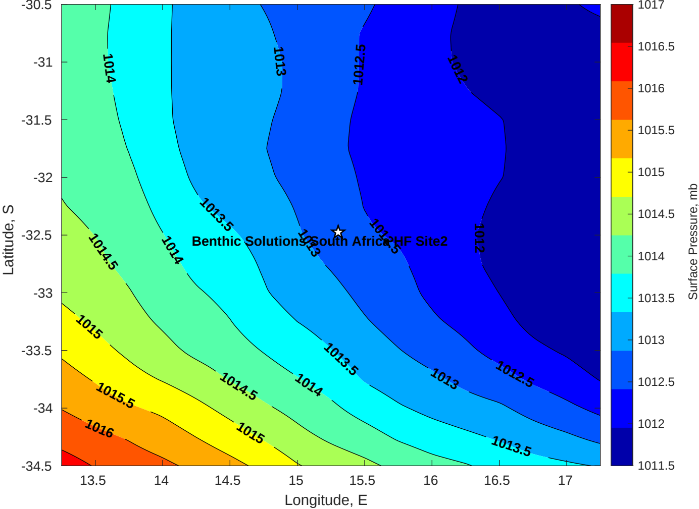
Surface Pressure (mb) for Benthic Solutions South Africa HF Site2 at 05-Apr-2025 00:00:00
