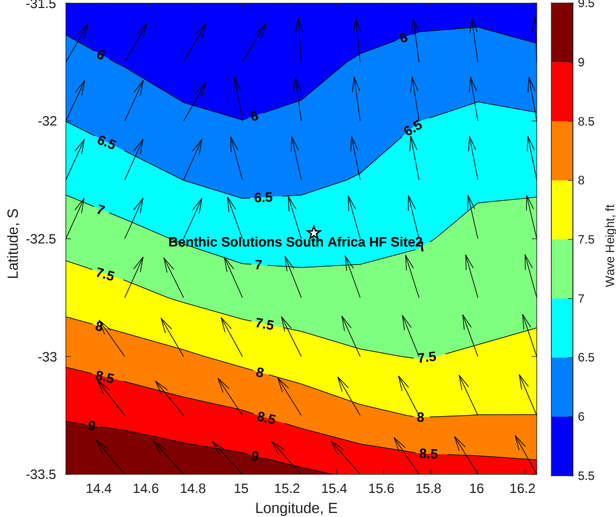
Wave Height (ft) for Benthic Solutions South Africa HF Site2 at 05-Apr-2025 09:00:00
