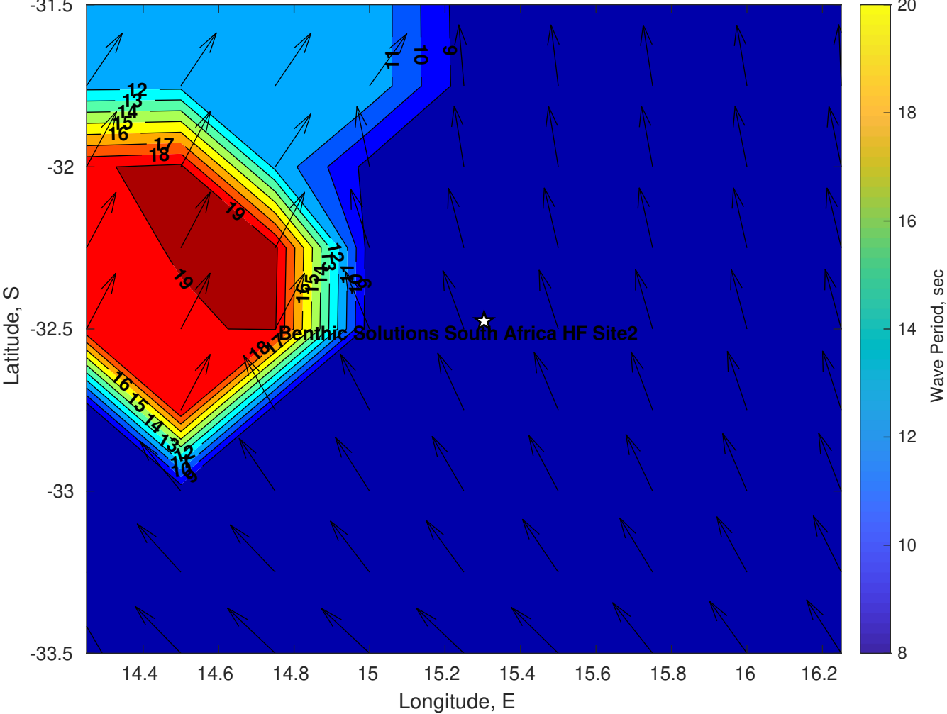
Wave Period (sec) for Benthic Solutions South Africa HF Site2 at 05-Apr-2025 09:00:00
