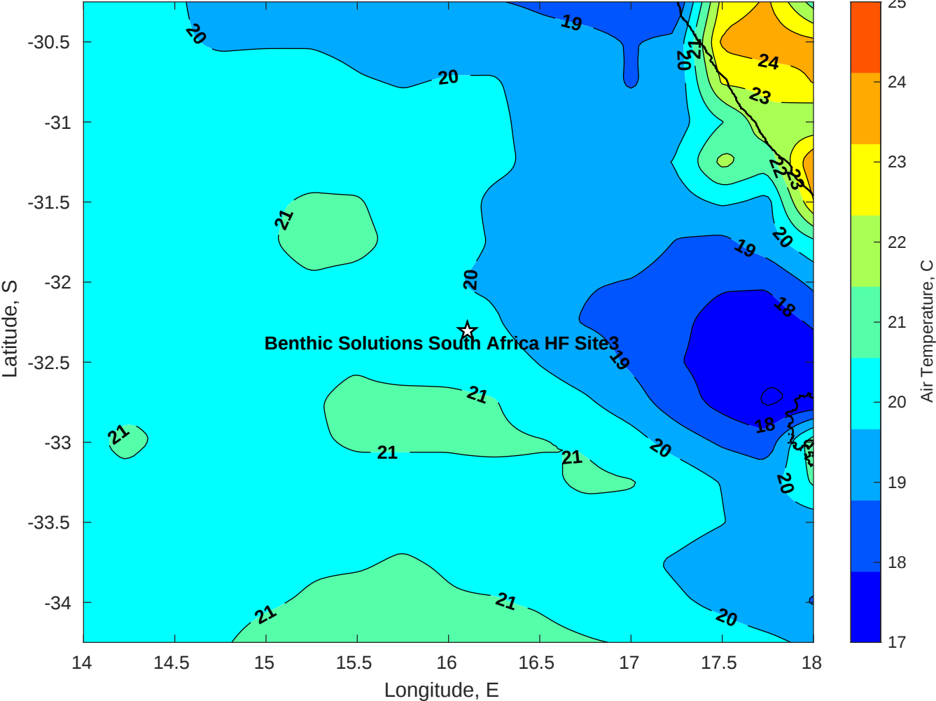
Air Temperature (C) for Benthic Solutions South Africa HF Site3 at 05-Apr-2025
