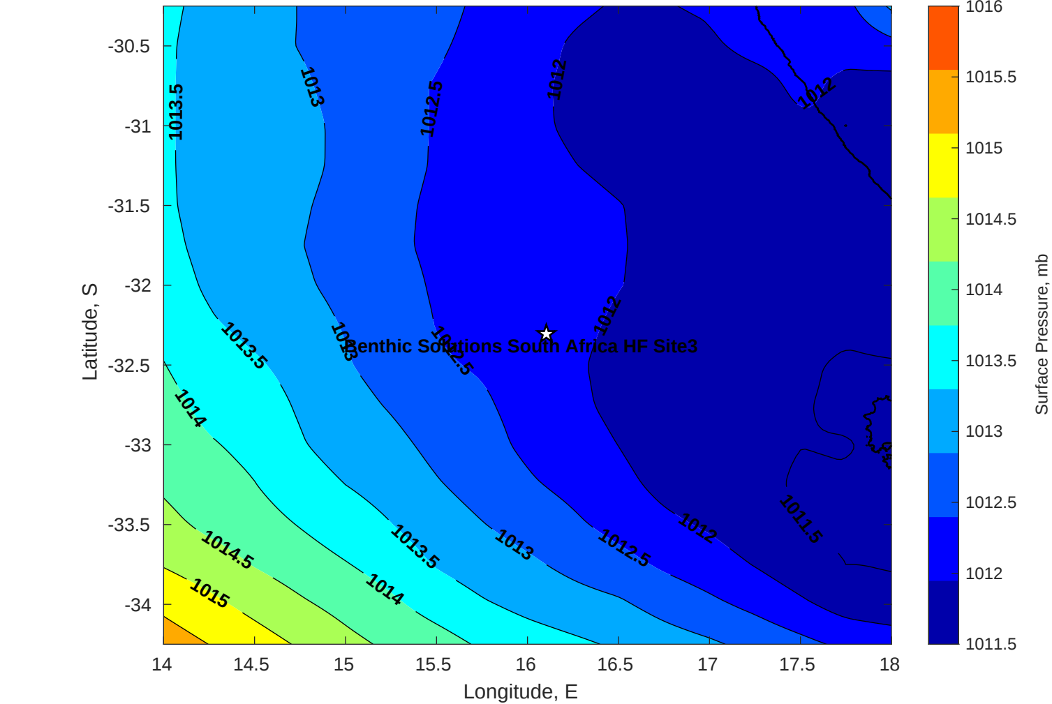
Surface Pressure (mb) for Benthic Solutions South Africa HF Site3 at 05-Apr-2025 00:00:00
