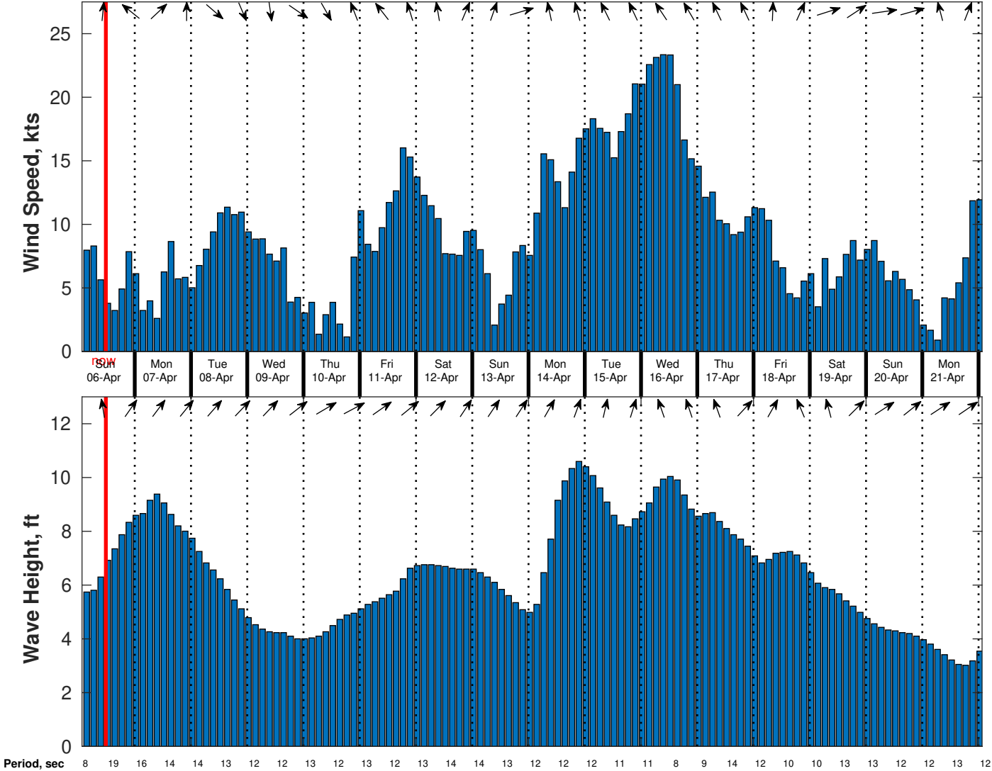
Wind & Wave Forecast for Benthic Solutions South Africa HF Site3 from 05-Apr-2025 02:00:00 to 21-Apr-2025 02:00:00
