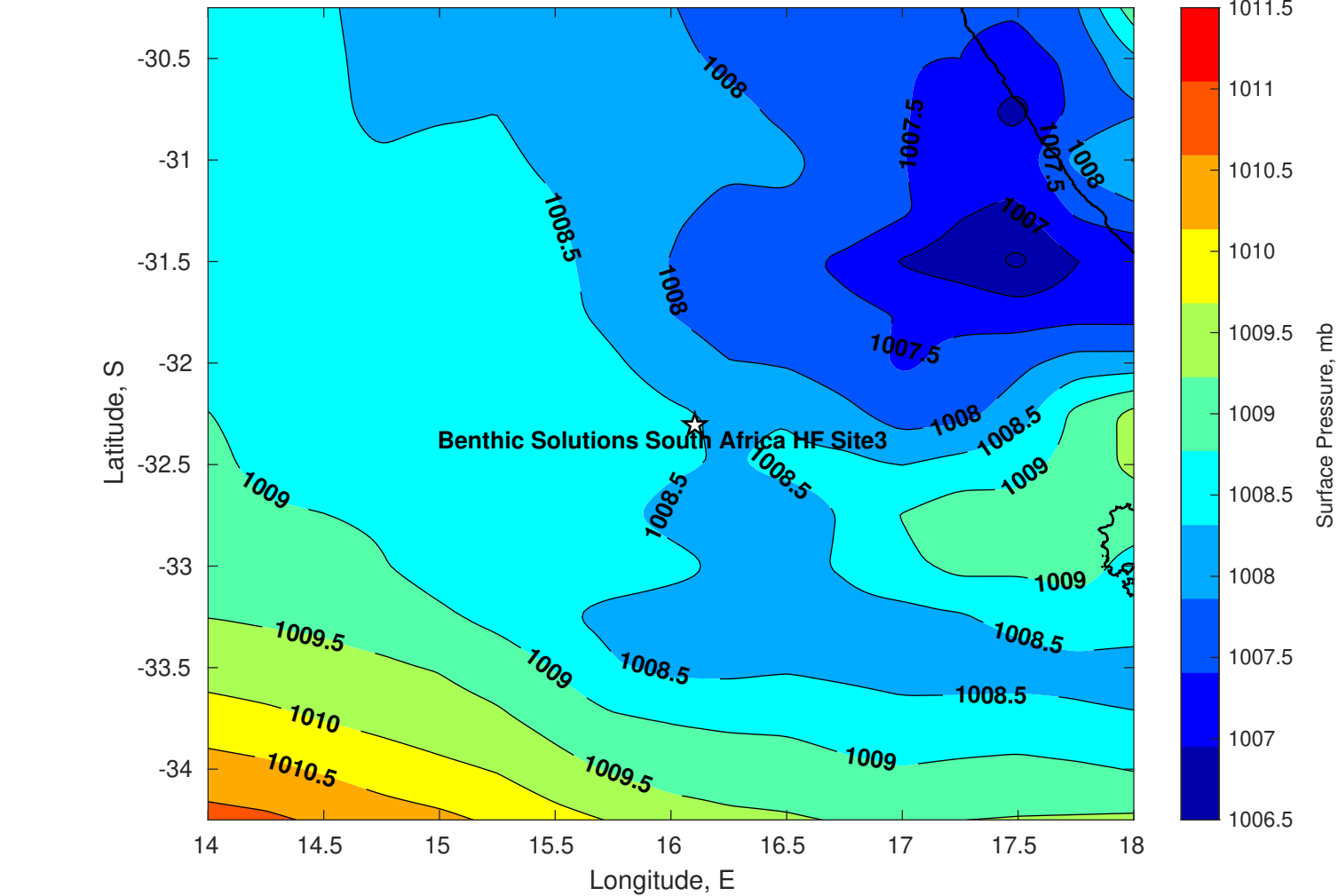
Surface Pressure (mb) for Benthic Solutions South Africa HF Site3 at 06-Apr-2025 00:00:00
