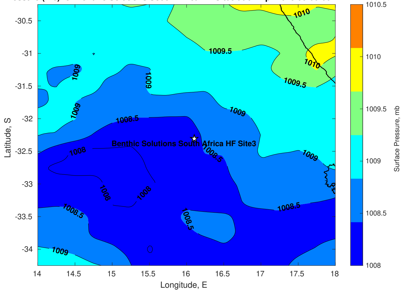
Surface Pressure (mb) for Benthic Solutions South Africa HF Site3 at 07-Apr-2025 00:00:00
