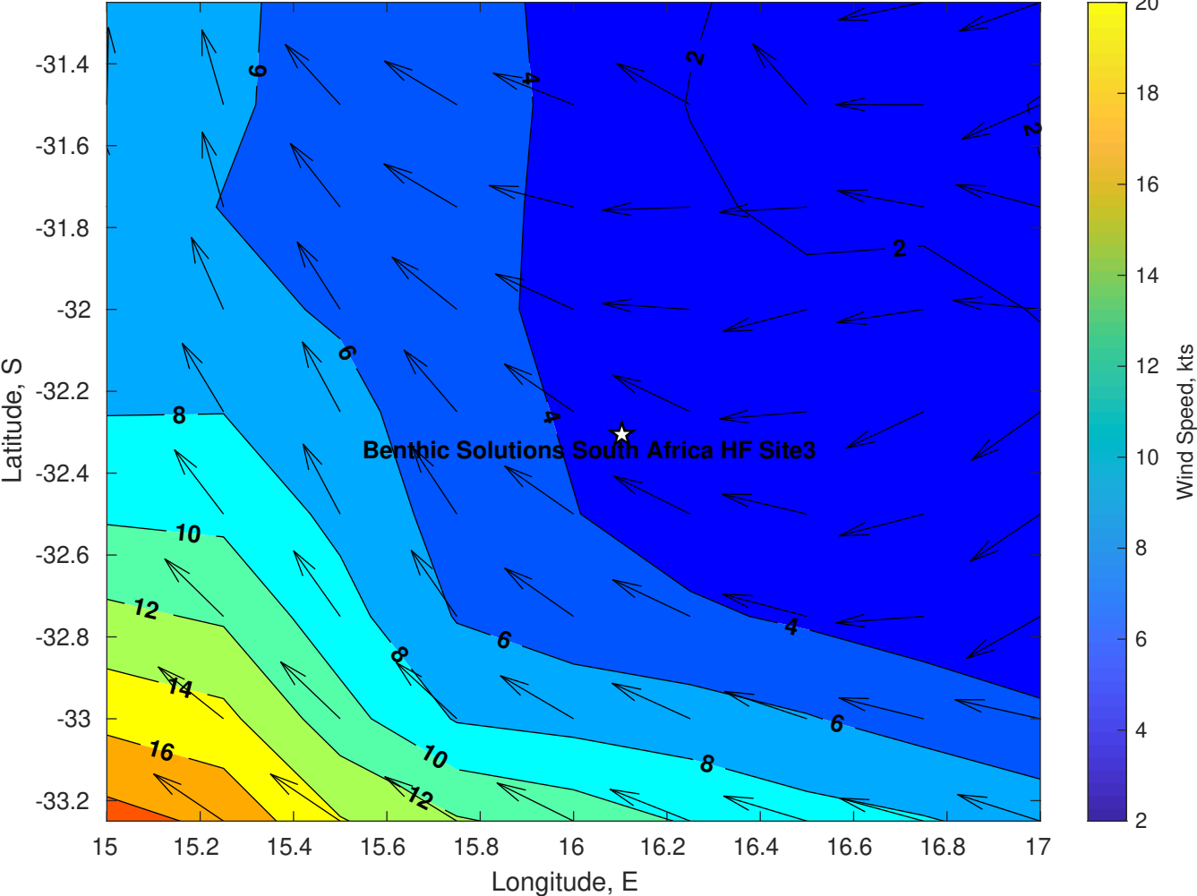
Winds (kts) for Benthic Solutions South Africa HF Site3 at 05-Apr-2025 09:00:00
