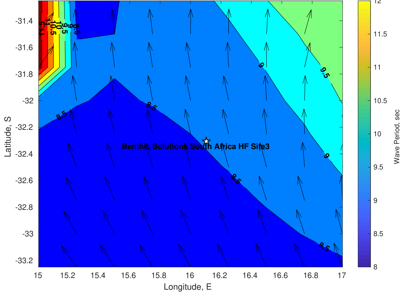
Wave Period (sec) for Benthic Solutions South Africa HF Site3 at 05-Apr-2025 09:00:00
