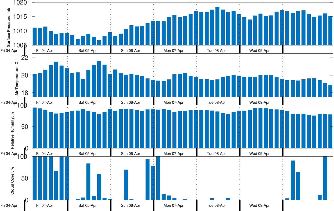
Met Forecast for Benthic Solutions South Africa HF Site3 from 05-Apr-2025 00:00:00 to 12-Apr-2025 00:00:00
