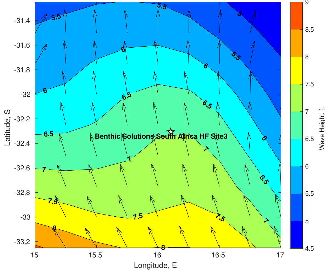
Wave Height (ft) for Benthic Solutions South Africa HF Site3 at 05-Apr-2025 09:00:00
