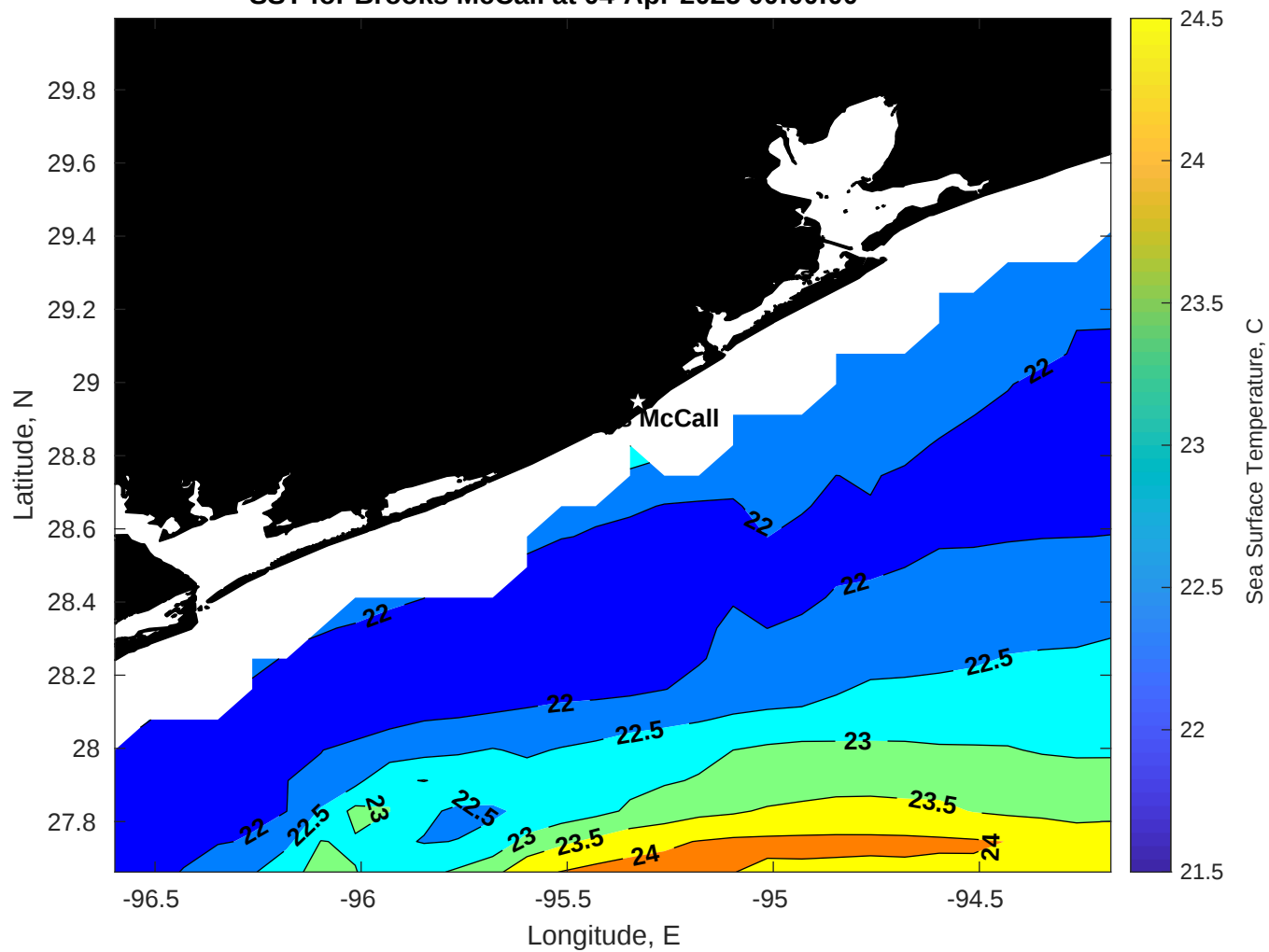
SST for Brooks McCall at 04-Apr-2025 00:00:00
