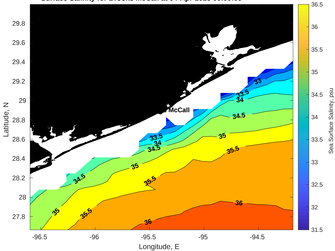
Surface Salinity for Brooks McCall at 04-Apr-2025 00:00:00
