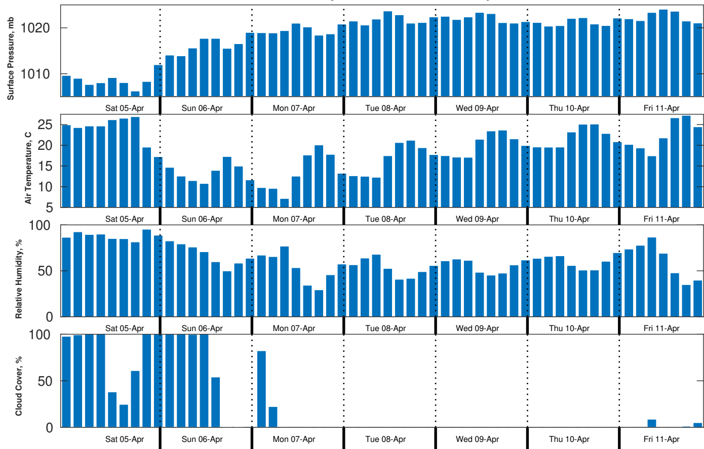
Met Forecast for Brooks McCall from 05-Apr-2025 00:00:00 to 12-Apr-2025 00:00:00
