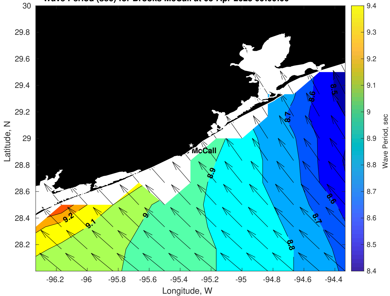
Wave Period (sec) for Brooks McCall at 05-Apr-2025 09:00:00
