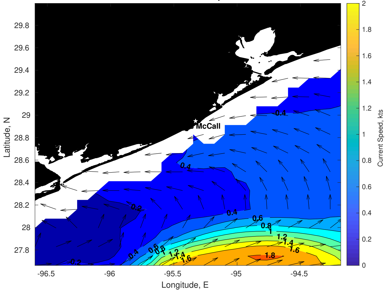
Surface Currents for Brooks McCall at 04-Apr-2025 00:00:00
