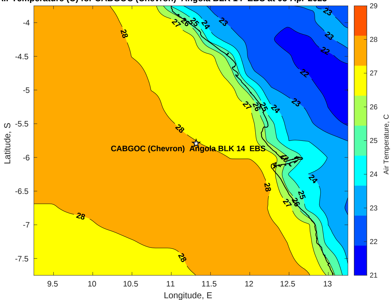
Air Temperature (C) for CABGOC (Chevron) Angola BLK 14 EBS at 05-Apr-2025
