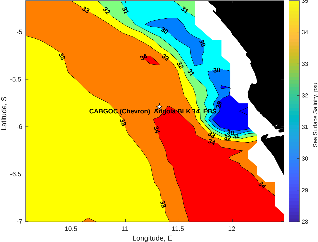
Surface Salinity for CABGOC (Chevron) Angola BLK 14 EBS at 04-Apr-2025 00:00:00
