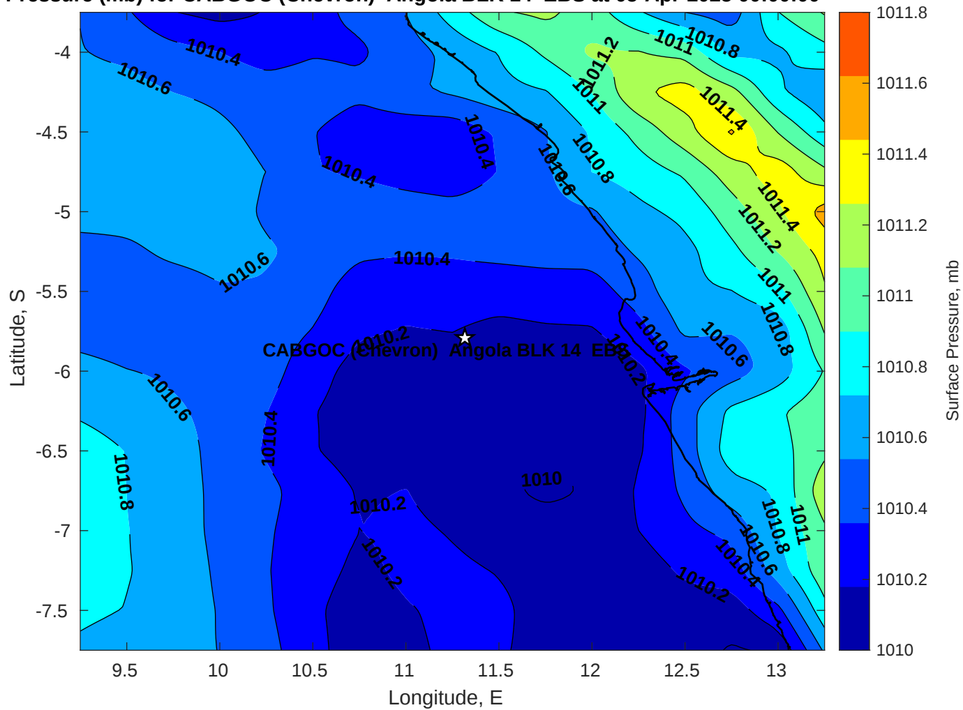
Surface Pressure (mb) for CABGOC (Chevron) Angola BLK 14 EBS at 05-Apr-2025 00:00:00
