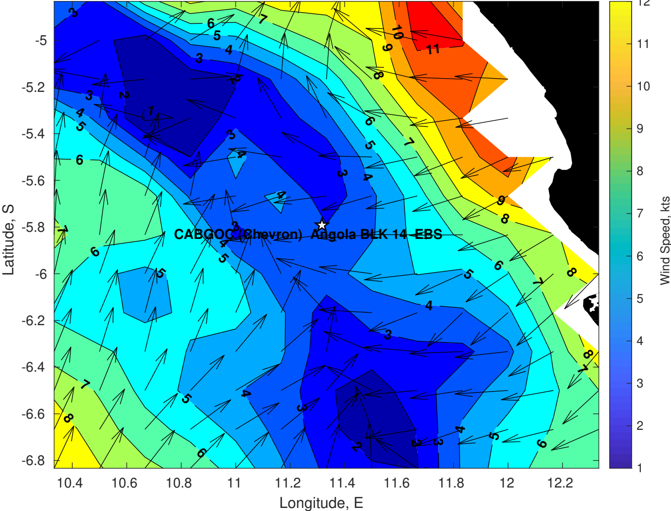
Winds (kts) for CABGOC (Chevron) Angola BLK 14 EBS at 05-Apr-2025 09:00:00
