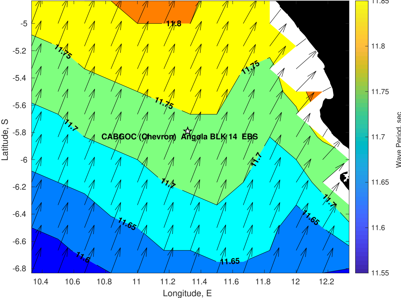
Wave Period (sec) for CABGOC (Chevron) Angola BLK 14 EBS at 05-Apr-2025 09:00:00
