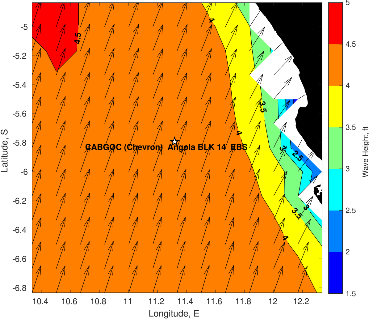
Wave Height (ft) for CABGOC (Chevron) Angola BLK 14 EBS at 05-Apr-2025 09:00:00
