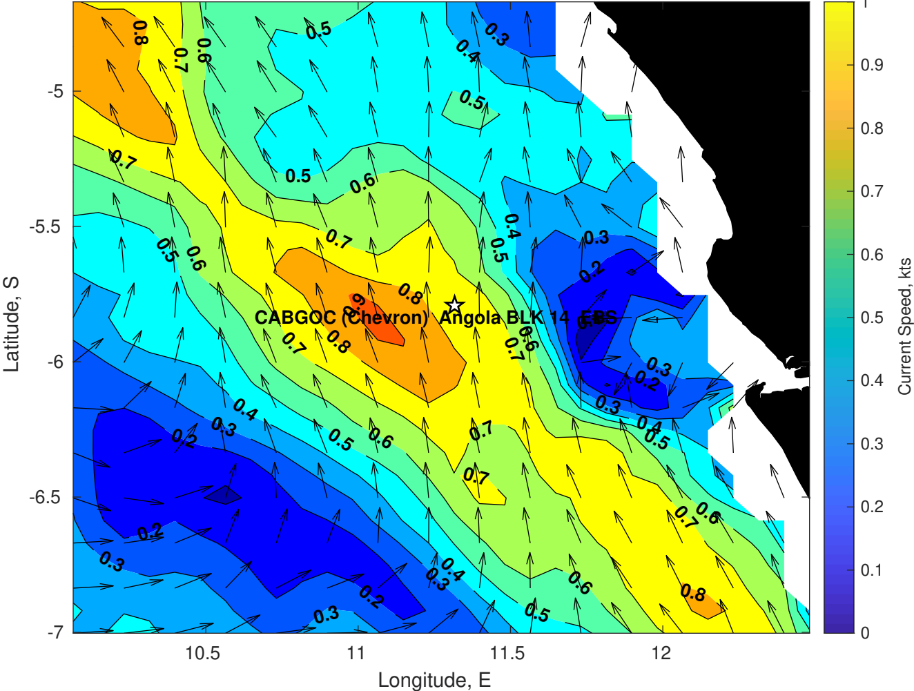
Surface Currents for CABGOC (Chevron) Angola BLK 14 EBS at 04-Apr-2025 00:00:00
