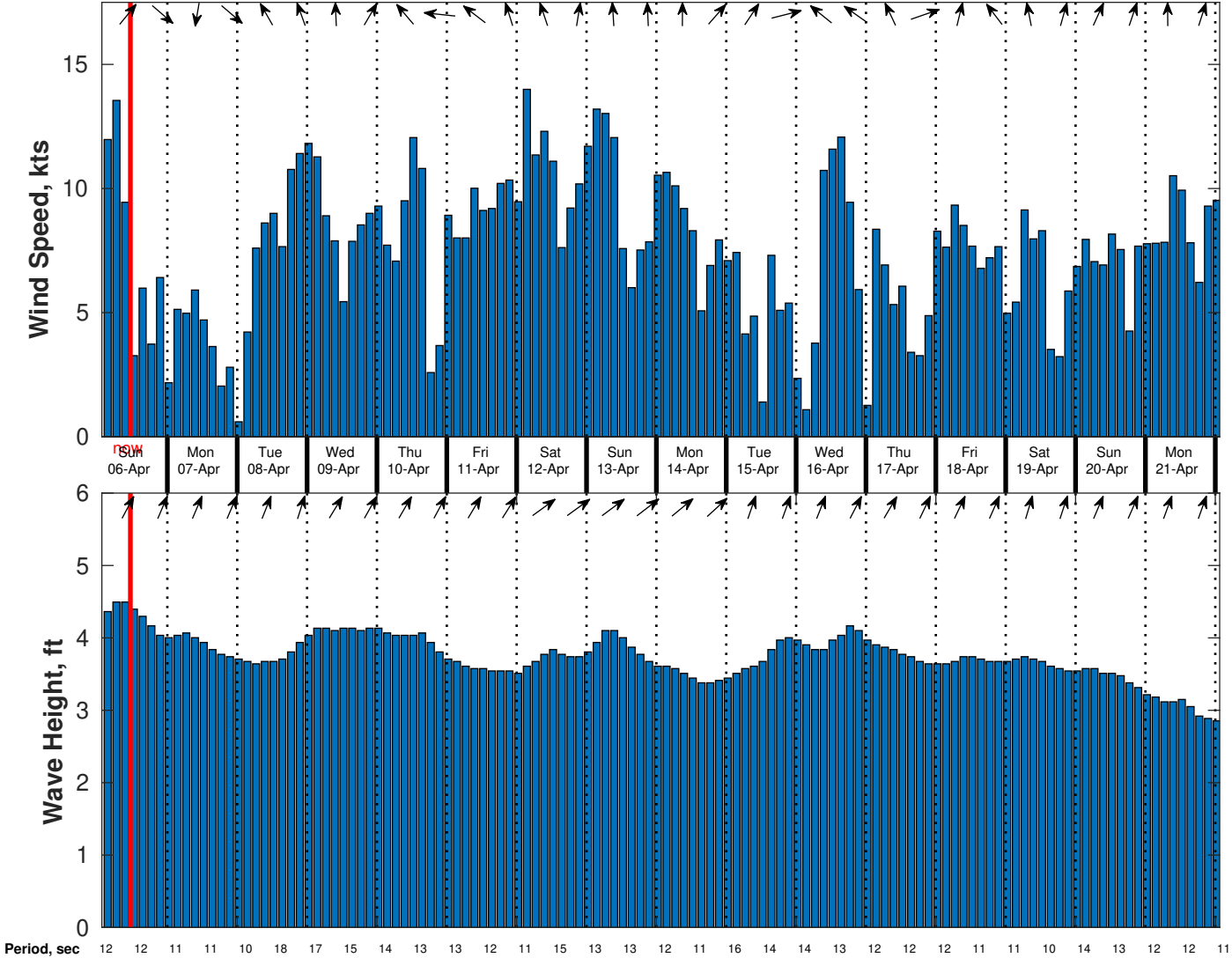
Wind & Wave Forecast for CABGOC (Chevron) Angola BLK 14 EBS from 05-Apr-2025 02:00:00 to 21-Apr-2025 02:00:00
