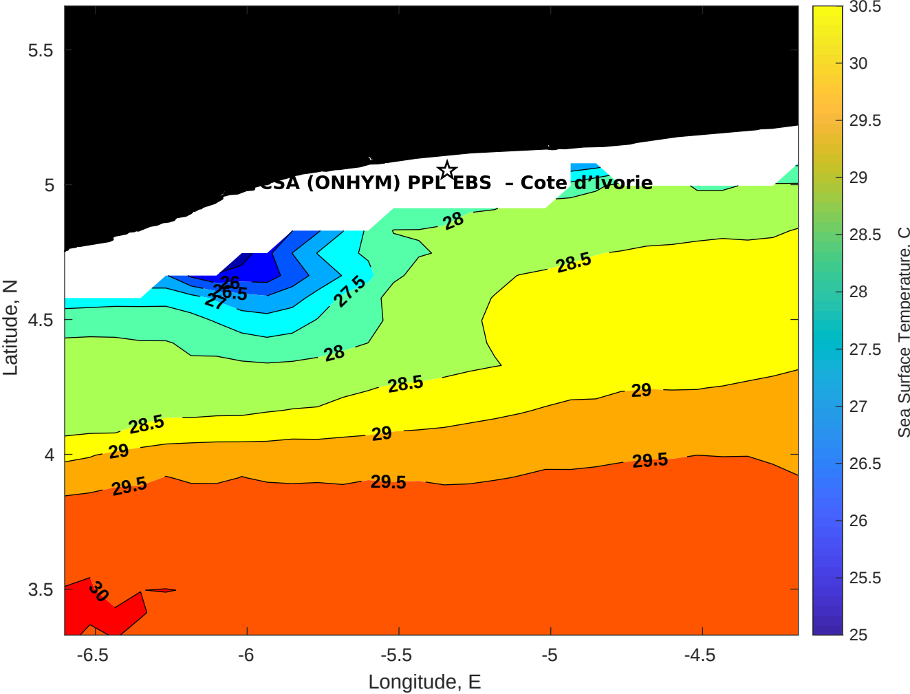
SST for CSA (ONHYM) PPL EBS - Cote d'Ivoire at 04-Apr-2025 00:00:00
