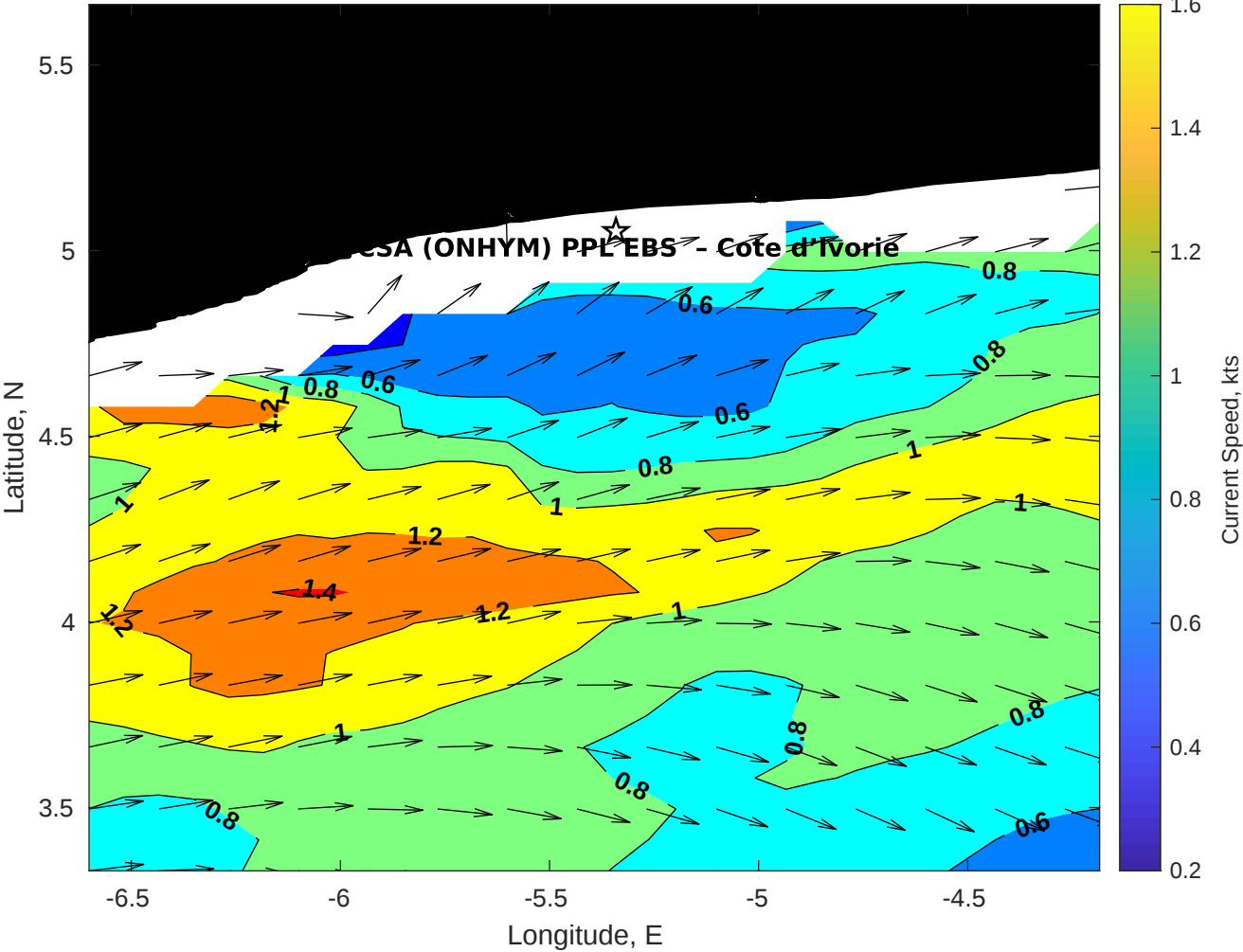
Surface Currents for CSA (ONHYM) PPL EBS - Cote d'Ivoire at 04-Apr-2025 00:00:00
