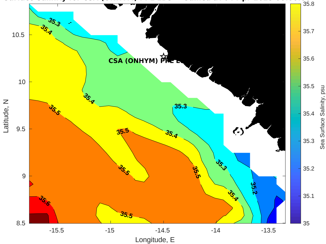
Surface Salinity for CSA (ONHYM) PPL EBS - Guinea at 04-Apr-2025 00:00:00
