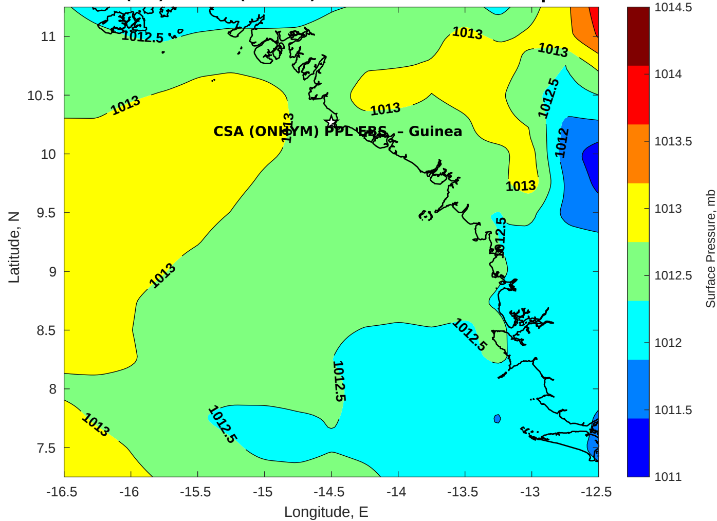
Surface Pressure (mb) for CSA (ONHYM) PPL EBS - Guinea at 05-Apr-2025 00:00:00
