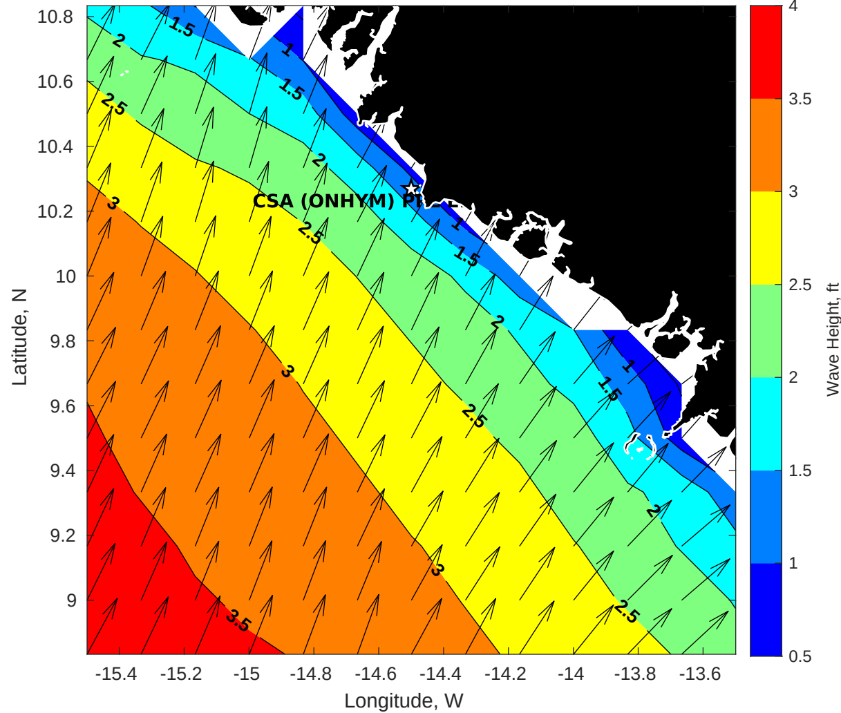
Wave Height (ft) for CSA (ONHYM) PPL EBS - Guinea at 05-Apr-2025 09:00:00
