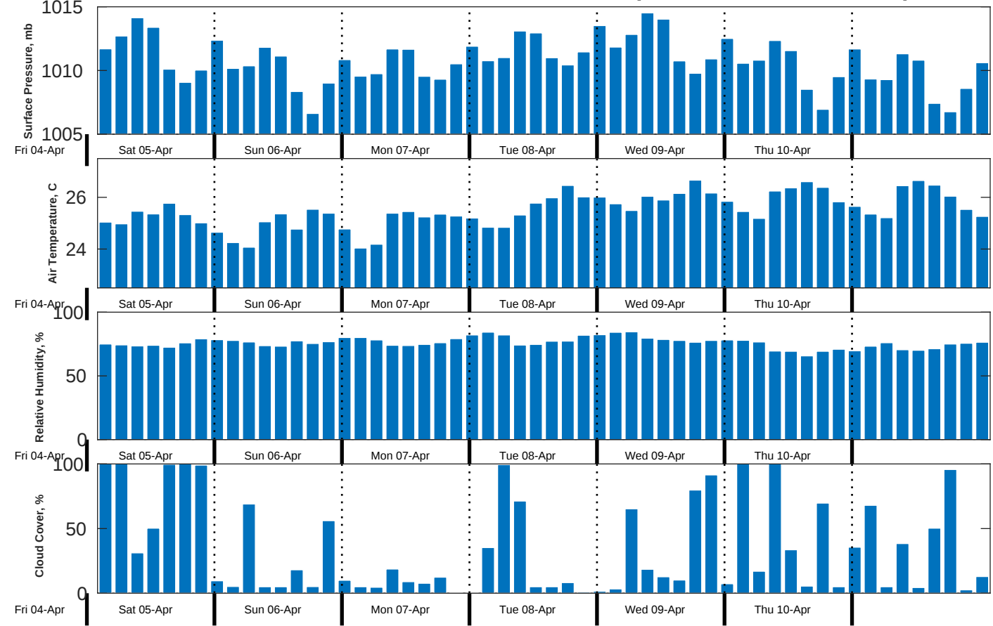
Met Forecast for CSA (ONHYM) PPL EBS - Guinea from 05-Apr-2025 00:00:00 to 12-Apr-2025 00:00:00
