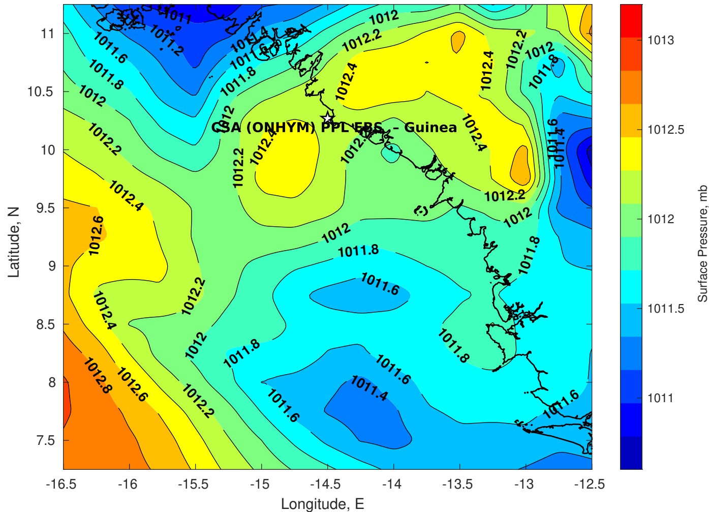
Surface Pressure (mb) for CSA (ONHYM) PPL EBS - Guinea at 06-Apr-2025 00:00:00
