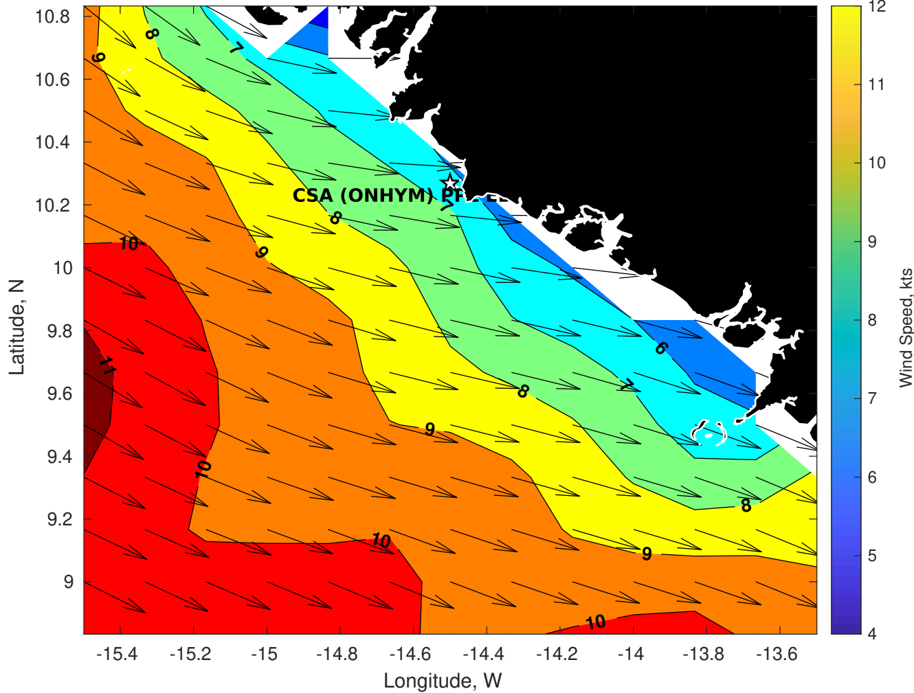
Winds (kts) for CSA (ONHYM) PPL EBS - Guinea at 05-Apr-2025 09:00:00
