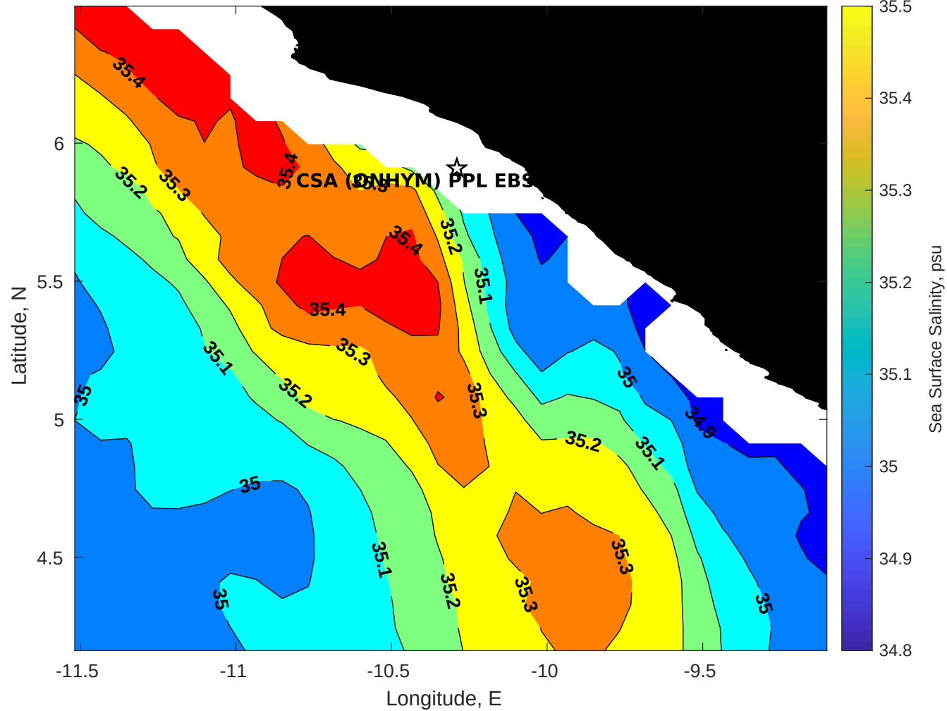
Surface Salinity for CSA (ONHYM) PPL EBS - Liberia at 04-Apr-2025 00:00:00
