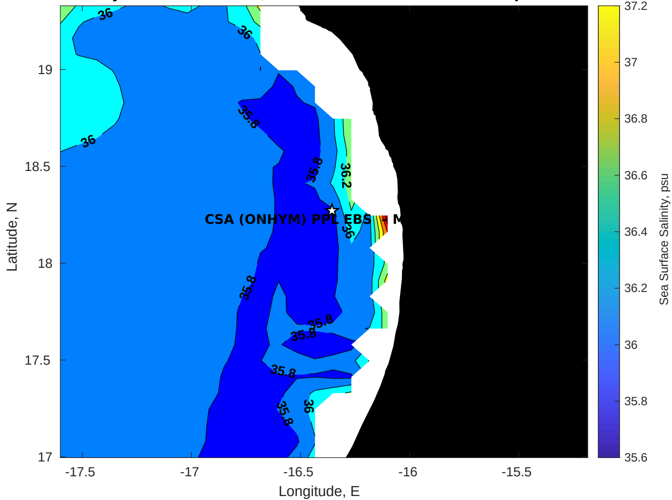
Surface Salinity for CSA (ONHYM) PPL EBS - Mauritania at 04-Apr-2025 00:00:00
